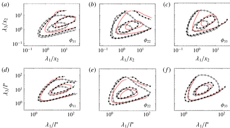
FIGURE 4. (Colour online) Premultiplied streamwise \phi_{11} (a,d), wall-normal \phi_{22} (b,e) and spanwise \phi_{33} (c,f) velocity two-dimensional spectra at x_2 = 0.10h for NS550 (—), NS550-s1 (○) and NS550-s2 (●). The wavelengths are scaled by x_2 in (a–c) and by l^* in (d–f). Contours are 0.1 and 0.6 of the maximum.
