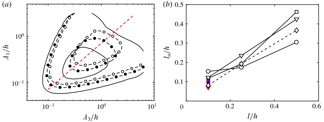
FIGURE 11. (Colour online) (a) Wall-parallel premultiplied boundary-normal velocity spectra at x_2^+ = 0 for R550 (—), R550-11 (○) and R550-12 (●). Contours are 0.1 and 0.6 of the maximum. The red dashed line is \lambda_3 = 0.7\lambda_1 . (b) Adaptation length l_a for the mean velocity profile (◇), and r.m.s. streamwise (○), boundary-normal (□) and spanwise (▽) velocity fluctuations as a function of the slip length l . Colours are black for R550, blue for R950 and red for R2000.
