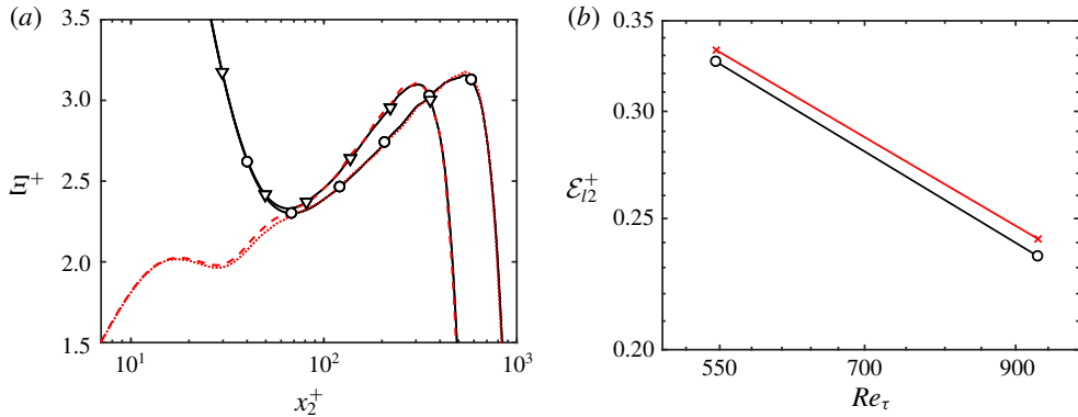
FIGURE 19. (Colour online) (a) Diagnostic function \mathcal{E} = x_2 \partial \langle u_1 \rangle / \partial x_2 for NS550 ( \nabla ), NS950 ( \circ ), R550-lplus (---) and R950-lplus ( \cdots ). (b) Plot of \mathcal{E}_{l2} as a function of Re_\tau for wall-bounded cases NS550 and NS950 ( \circ ), and Robin-bounded cases R550-lplus and R950-lplus ( \times ).
