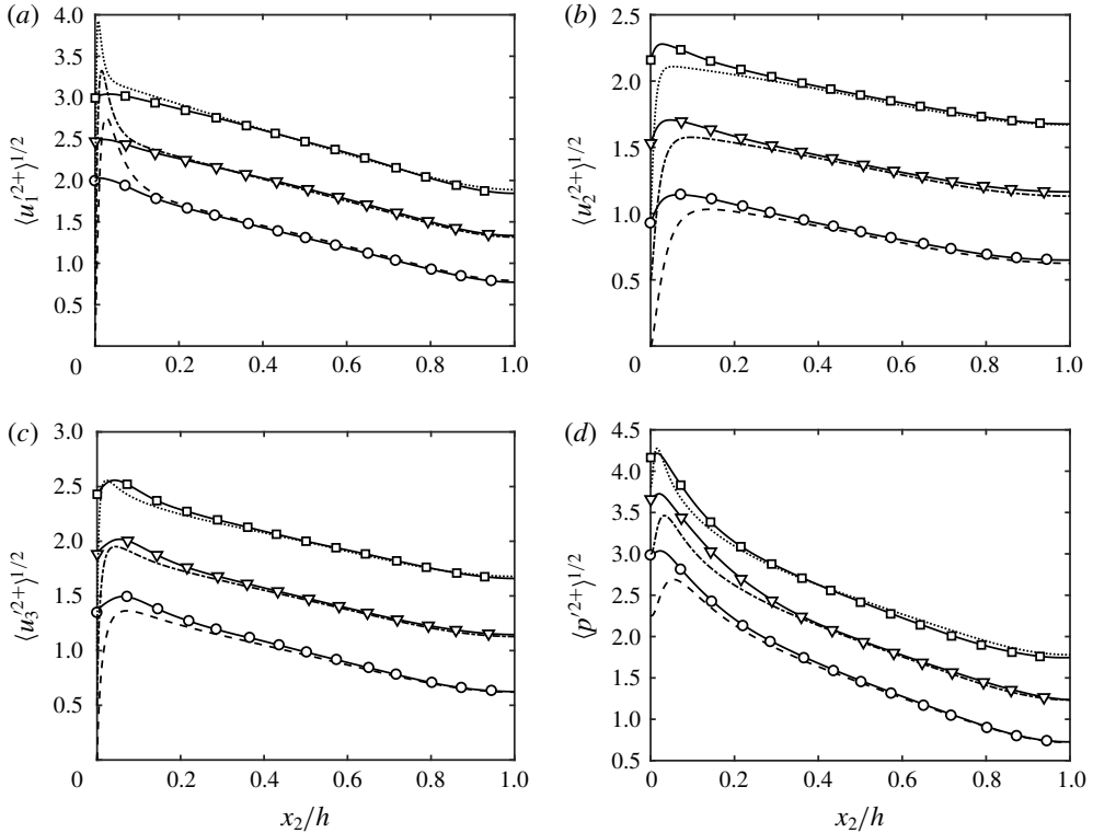
FIGURE 9. (a) Streamwise, (b) wall-normal (or boundary-normal) and (c) spanwise r.m.s. velocity fluctuations, and (d) r.m.s. pressure fluctuations for R550 ( \circ ), R950 ( \nabla ), R2000 ( \square ), NS550 (---), NS950 (-·-·-) and NS2000 (·····). In all panels, the profiles for cases at Re_\tau \approx 950 and Re_\tau \approx 2000 are vertically shifted by 0.5 and 1 plus units, respectively, for clarity.
