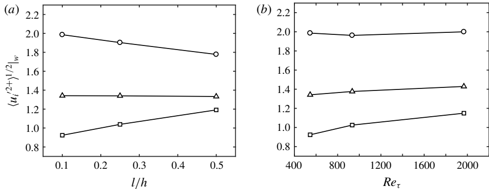
FIGURE 17. Streamwise (O), wall-normal (□) and spanwise (Δ) r.m.s. fluctuating velocities at x_2/h = 0 for Robin-bounded cases as a function of (a) slip length and (b) friction Reynolds number.
