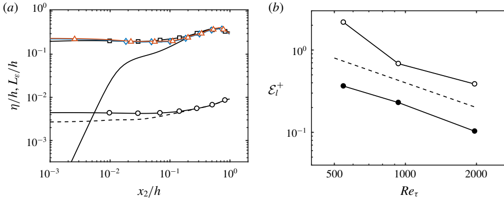
FIGURE 12. (Colour online) (a) Kolmogorov length scale \eta for NS550 (---) and R550 ( \circ ), and integral length scale L_\varepsilon for NS550 (—), R550 ( \square ), R950 ( \diamond ) and R2000 ( \triangle ). (b) \varepsilon_l^+ as a function of Re_\tau . Closed and open symbols are for wall-bounded and Robin-bounded cases, respectively. The dashed line is \varepsilon_l^+ \sim Re_\tau^{-1} .
