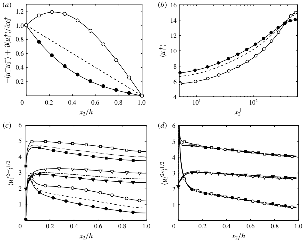
FIGURE 2. Mean (a) total tangential Reynolds stress and (b) streamwise velocity profile for NS550 (---), NS550-p (○) and NS550-n (●). Panels (c,d) contain the streamwise (circles and ---), wall-normal (triangles and - · - · -) and spanwise (squares and · · · · ·) r.m.s. velocity fluctuations scaled with (c) u_\tau and (d) u^* . Symbols are for NS550-p (open) and NS550-n (closed). Lines without symbols are for NS550. For clarity, the profiles for the wall-normal and spanwise r.m.s. velocity fluctuations are shifted vertically by 2.0 and 3.4 wall units.
