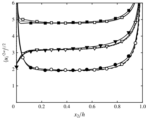
FIGURE 15. Streamwise (circles and ---), wall-normal (triangles and ---) and spanwise (squares and ·····) r.m.s. velocity fluctuations scaled with u^* . Symbols are for NS550-p (open) and NS550-n (closed). Lines without symbols are for NS550. For clarity, the profiles for the wall-normal and spanwise r.m.s. velocity fluctuations are shifted vertically by 2.0 and 3.4 wall units.
