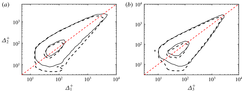
FIGURE 14. (Colour online) Joint p.d.f.s of the logarithms of the box sizes of structures, (a) p(\Delta_1^+, \Delta_2^+) and (b) p(\Delta_3^+, \Delta_2^+) , for NS2000 (—) and R2000 (---). Contours contain 50% and 99.8% of the p.d.f. The dashed straight lines are \Delta_1 = 1.5\Delta_2 and \Delta_1 = \Delta_3 , respectively.
