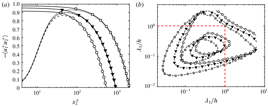
FIGURE 6. (Colour online) (a) Mean tangential Reynolds stress as a function of the wall-normal (or boundary-normal) coordinate for R550 (○), R950 (▼), R2000 (□), NS550 (---), NS950 (-·-·-) and NS2000 (· · · · ·). (b) Premultiplied boundary-normal two-dimensional velocity spectra for Robin-bounded channels at x_2/h = 0 . Contours are 0.1 and 0.6 of the maximum. The red dashed lines are \lambda_1/h = 1 and \lambda_3/h = 1 . Symbols are as in panel (a).
