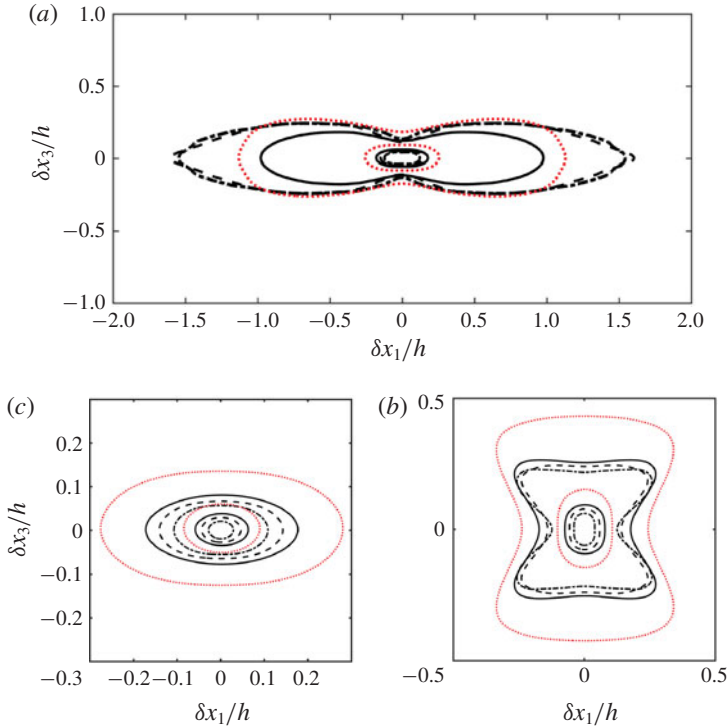
FIGURE 18. (Colour online) Wall-parallel ( x_1 – x_3 ) correlations of the (a) streamwise, (b) wall-normal and (c) spanwise velocity for R550 (—), R950 (---), R2000 (— · —) and R550-11 (·····). Contours are 0.05 and 0.5 of the maximum value. The mean flow is from left to right.
