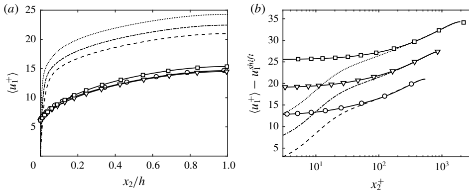
FIGURE 8. Mean streamwise velocity profiles as a function of x_2 in (a) linear scale and (b) logarithmic scale for R550 ( \circ ), R950 ( \nabla ), R2000 ( \square ), NS550 (---), NS950 (----) and NS2000 ( \cdots ). In panel (b), the velocity profiles of Robin-bounded cases are vertically shifted such that the centreline velocity coincides with their corresponding wall-bounded case. For clarity, profiles at Re_\tau \approx 950 and Re_\tau \approx 2000 are additionally shifted by 5 and 10 plus units, respectively.
