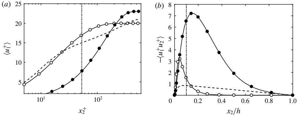
FIGURE 3. Mean (a) streamwise velocity profile and (b) tangential Reynolds stress for NS550 (---), NS550-s1 (○) and NS550-s2 (●). The dash-dotted line is x_2 = 0.1h .
