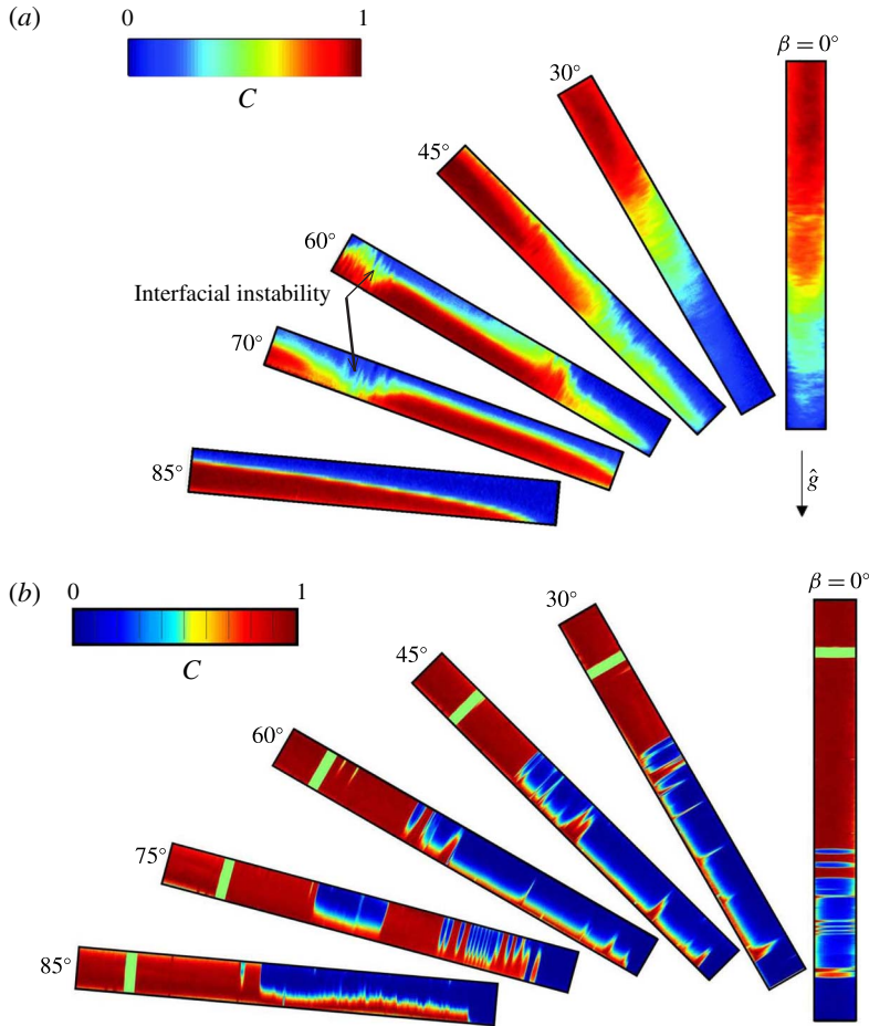
FIGURE 6. (Colour online) Change in iso-viscous displacement flow with \beta . (a) For miscible fluids (salt-water displacing water) of Alba et al. (2013a) ( At=0.0035 , Re \approx 726 , Fr \approx 1.48 , Ca = \infty ). The field of view is 1330 \times 19.05 \text{ mm}^2 located 1740 \text{ mm} downstream of the gate valve. (b) For immiscible fluids (current study) obtained for \hat{\rho}_H = 1181 \text{ kg m}^{-3} , \hat{\rho}_L = 918 \text{ kg m}^{-3} and approximately close imposed flow rates \hat{V}_0 \in [71, 114] \text{ mm s}^{-1} ( At=0.125 , Re \in [146, 247] , Fr \in [0.66, 1.05] , Ca \in [0.06, 0.25] , \theta = 56^\circ ). The field of view is 1750 \times 9.53 \text{ mm}^2 . The colour bar at the top left of the figures shows the corresponding concentration value, C , with 0 referring to the pure displaced fluid and 1 to the pure displacing fluid.
