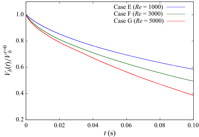
Figure 22. Volume ratio vs time for a dissolving bubble in a TC device at different rotating speeds. Gravity is not taken into account.
