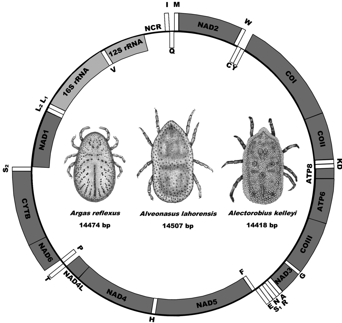
Fig. 1. Mitochondrial genome arrangement for Alveonasus lahorensis , Argas reflexus and Alectorobius kelleyi . Genes on the outside are on the forward strand whereas genes on the inside are on the reverse or complementary strand. Protein-encoding genes are in dark grey, ribosomal genes in light grey whereas transfer RNA genes are in white boxes. Also indicated are mitochondrial genome sizes.
