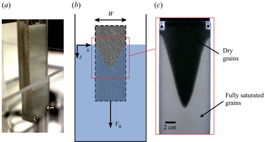
Figure 2. (a) Photo of the porous medium made of grains (system W3). The front and rear are made of PMMA, and the sides and bottom of the cell consist of a metal wire mesh with openings of 250\ \mu\text{m} . (b) Schematic of the experimental set-up. A vertical linear motor imposes the speed of translation V_0 . (c) Picture of the stationary impregnation front during the translation of the porous medium into the water bath. The system is illuminated by an LED panel placed behind the cell. The light part is fully saturated with water whereas the dark part is dry.
