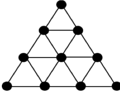
Figure 1. Pile of rocks represented as an undirected graph.
