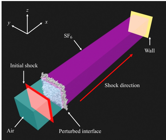
Figure 2. Sketch diagram of the computational setting and initial conditions of the RMI with reshock.
