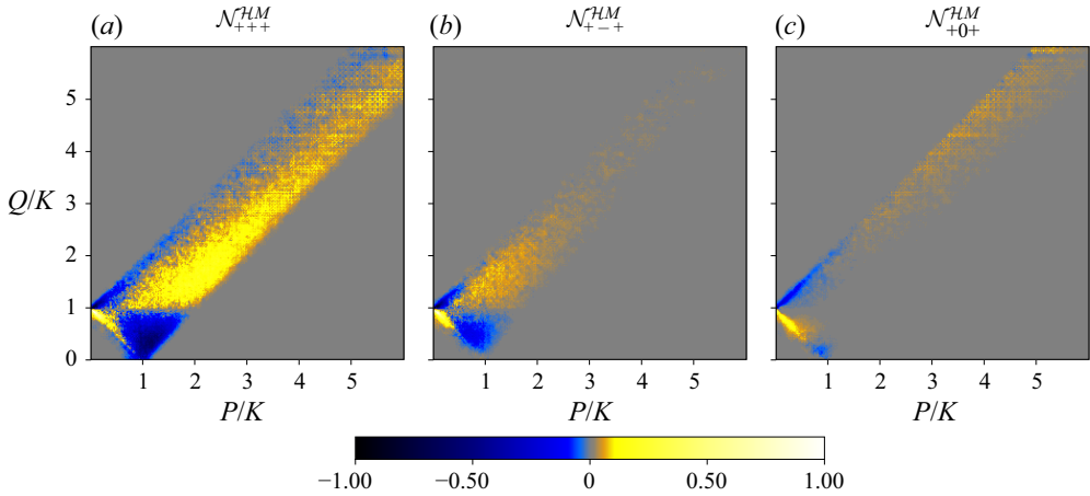
Figure 10. Average of the 46 slices of \mathcal{N}_{sk^sps_Q}^{\mathcal{H}^M}(Q, P, K_0) for K_0 \in [5, 50] , obtained through the procedure described in Appendix B . Each plot is normalised by its own maximum absolute value.
