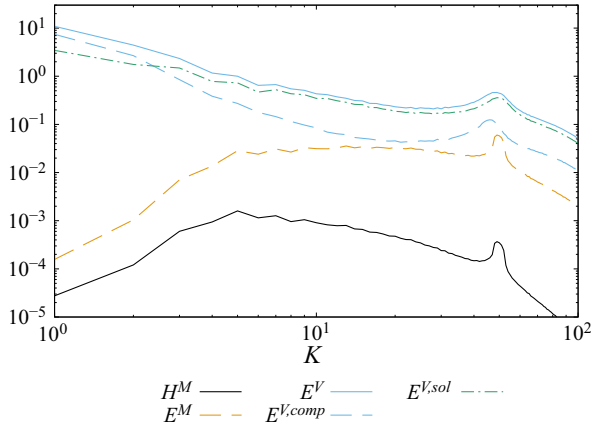
Figure 1. Magnetic helicity H^M , magnetic energy E^M and specific kinetic energy E^V spectra (decomposed into solenoidal E^{V,sol} = E^{V,+} + E^{V,-} and compressive E^{V,0} parts such that E^V = E^{V,sol} + E^{V,0} ) for the M8c run at an instant when \mathcal{T}_{\mathcal{H}^M} \approx L/10 .
