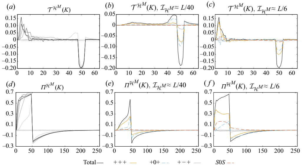
Figure 15. (a) Time evolution of the magnetic helicity transfer Fourier spectra \sum_{P,Q} T^{\mathcal{H}^M}(Q, P, K) for the M8c run; five snapshots equally spaced in time between instants when \mathcal{I}_{\mathcal{H}^M} \approx L/40 and \mathcal{I}_{\mathcal{H}^M} \approx L/6 . (b, c) Magnetic helicity transfer spectra at the extreme instants of panel (a) and some important helical contributions. (d–f) Same as (a–c) but with the magnetic helicity fluxes \Pi^{\mathcal{H}^M}(K) = \sum_{K_0=0}^K T^{\mathcal{H}^M}(K) .
