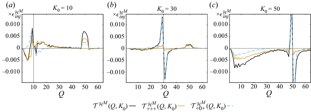
Figure 6. Cuts from the two-dimensional plots of figure 5 for K_0 \in \{10, 30, 50\} . The horizontal dotted line corresponds to y = 0 and the vertical one to Q = K_0 .
