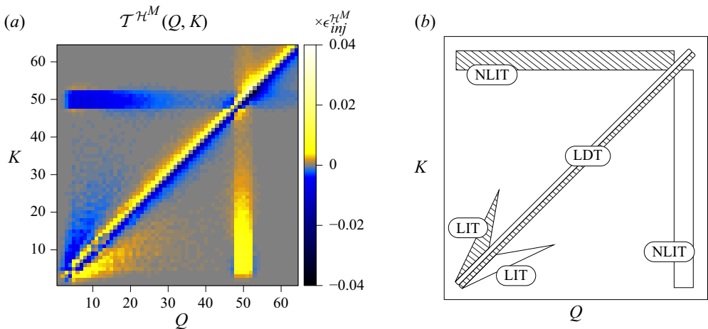
Figure 2. (a) Magnetic helicity transfer rates from shell Q to shell K for the M8c run, at an instant when \mathcal{T}_{\mathcal{H}^M} \approx L/10 . (b) Sketch of these transfer rates explicitly showing the non-local inverse transfer (NLIT), the local transfer (LIT) and the local direct transfer (LDT).
