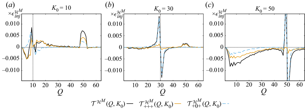
Figure 6. Cuts from the two-dimensional plots of figure 5 for K_0 \in \{10, 30, 50\} . The horizontal dotted line corresponds to y = 0 and the vertical one to Q = K_0 .
