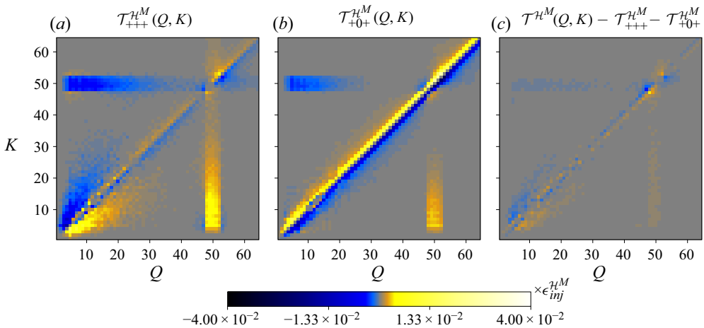
Figure 5. Contributions from the +++ and +0+ terms to the magnetic helicity transfer rates for the M8c run, at an instant when \mathcal{I}_{\mathcal{H}^M} \approx L/10 . Their sum is close to the total transfer function from figure 2 and the remaining contributions come mostly from the terms shown in figure 7.
