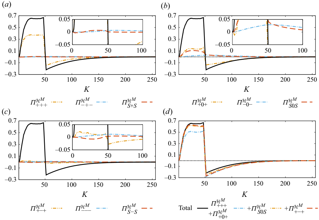
Figure 4. (a–c) The nine helically decomposed fluxes of magnetic helicity, compared to the total flux (in black), showing which ones are dominant, for the M8c run at an instant when \mathcal{I}_{\mathcal{H}^M} \approx L/10 . The plots are normalised by the magnetic helicity injection rate. The insets are zooms close to the horizontal \Pi^{\mathcal{H}^M} = 0 . (d) Comparison of successive sums of dominant terms.
