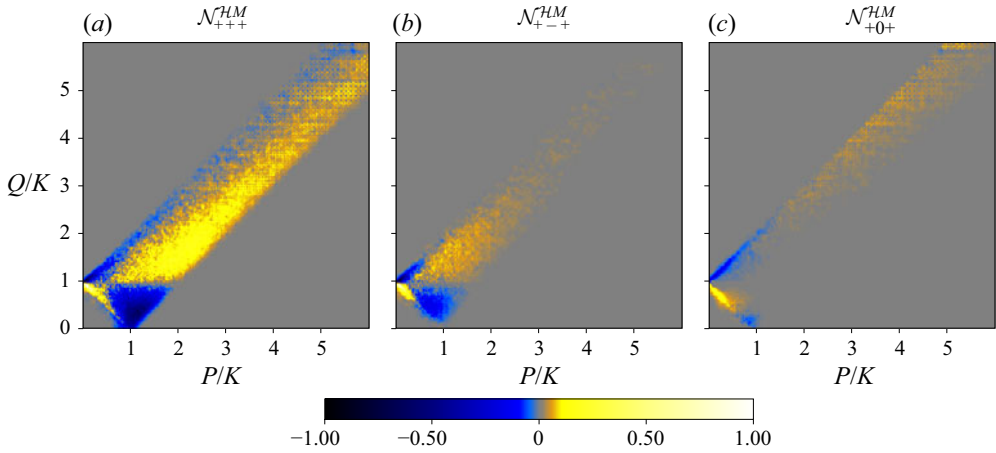
Figure 10. Average of the 46 slices of \mathcal{N}_{sk^s p^s Q}^{\mathcal{H}^M}(Q, P, K_0) for K_0 \in [5, 50] , obtained through the procedure described in Appendix B . Each plot is normalised by its own maximum absolute value.
