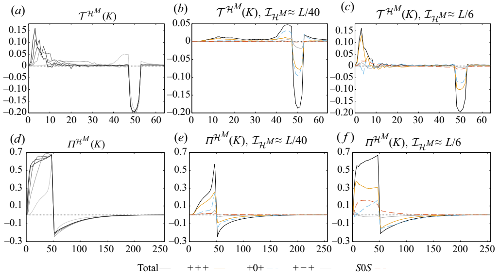
Figure 15. (a) Time evolution of the magnetic helicity transfer Fourier spectra \sum_{P,Q} \mathcal{T}^{\mathcal{H}^M}(Q, P, K) for the M8c run; five snapshots equally spaced in time between instants when \mathcal{I}_{\mathcal{H}^M} \approx L/40 and \mathcal{I}_{\mathcal{H}^M} \approx L/6 . (b, c) Magnetic helicity transfer spectra at the extreme instants of panel (a) and some important helical contributions. (d–f) Same as (a–c) but with the magnetic helicity fluxes \Pi^{\mathcal{H}^M}(K) = \sum_{K_0=0}^K \mathcal{T}^{\mathcal{H}^M}(K) .
