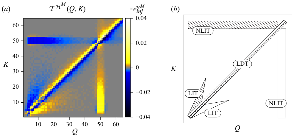
Figure 2. (a) Magnetic helicity transfer rates from shell Q to shell K for the M8c run, at an instant when \mathcal{I}_{\mathcal{H}^M} \approx L/10 . (b) Sketch of these transfer rates explicitly showing the non-local inverse transfer (NLIT), the local transfer (LIT) and the local direct transfer (LDT).
