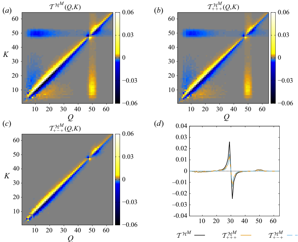
Figure 14. (a–c) Magnetic helicity transfer rates from shell Q to shell K for the M01s4 run at an instant when \mathcal{I}_{\mathcal{H}^M} \approx L/10 , as well as the biggest helical contributions. (d) Cuts of panels (a–c) at K_0 = 30 . The transfers are expressed in units of the magnetic helicity injection rate \epsilon_{inj}^{\mathcal{H}^M} .
