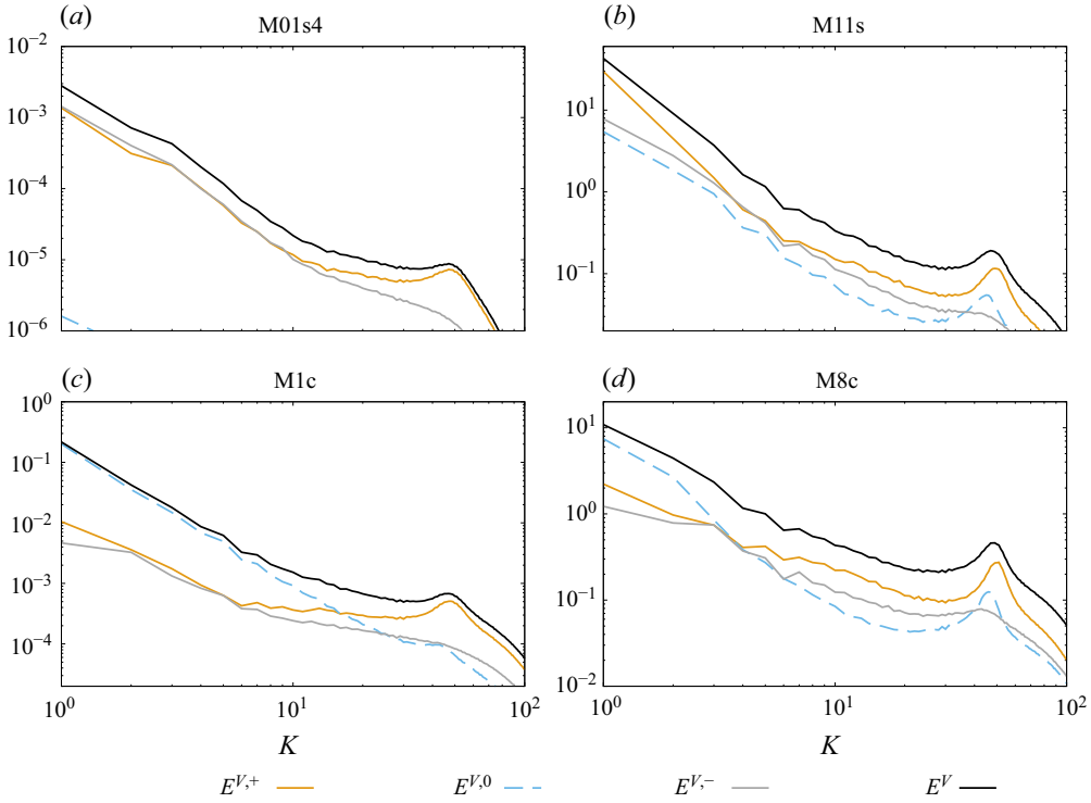
Figure 9. Repartition of the specific kinetic energy in the helical components for all the extreme runs, at an instant when \mathcal{T}_{\mathcal{H}^M} \approx L/10 .
