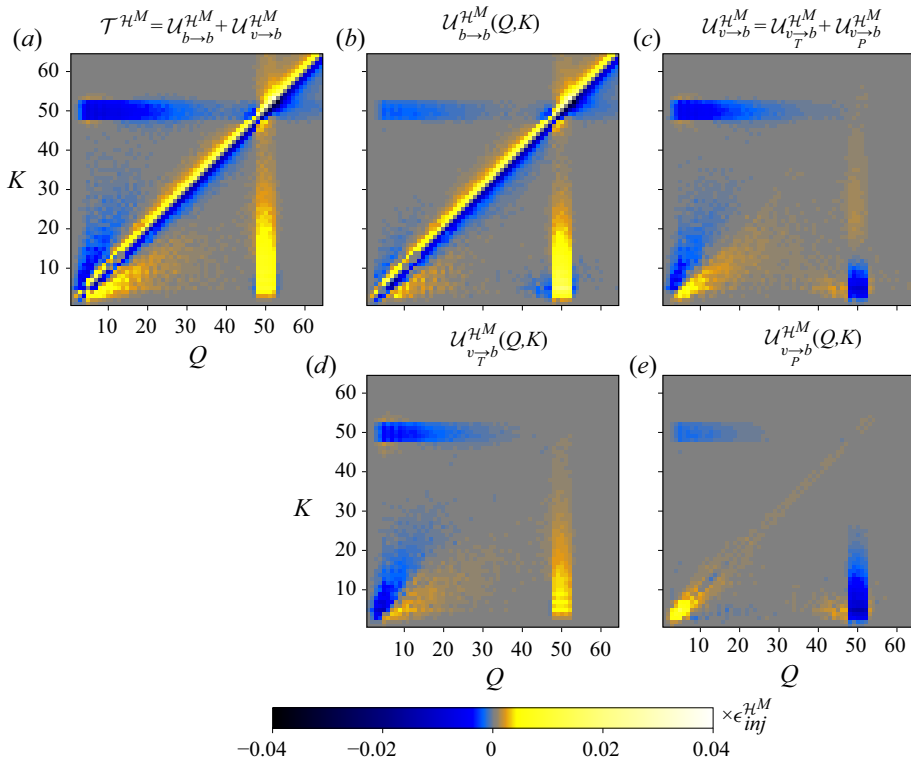
Figure 11. Decomposition of the magnetic helicity transfer rate from shell Q to shell K (panel (a), which is the same as figure 2 ) in different contributions: (b) associated with B \leftrightarrow B exchanges, (c) associated with V \leftrightarrow B exchanges, the latter being the sum of (d) contributions through the magnetic tension and (e) through the magnetic pressure.
