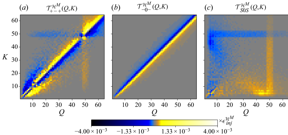
Figure 7. Contributions from the +-+ , -0- and S0S terms to the magnetic helicity transfer rates for the M8c run, at an instant when \mathcal{I}_{\mathcal{H}^M} \approx L/10 .
