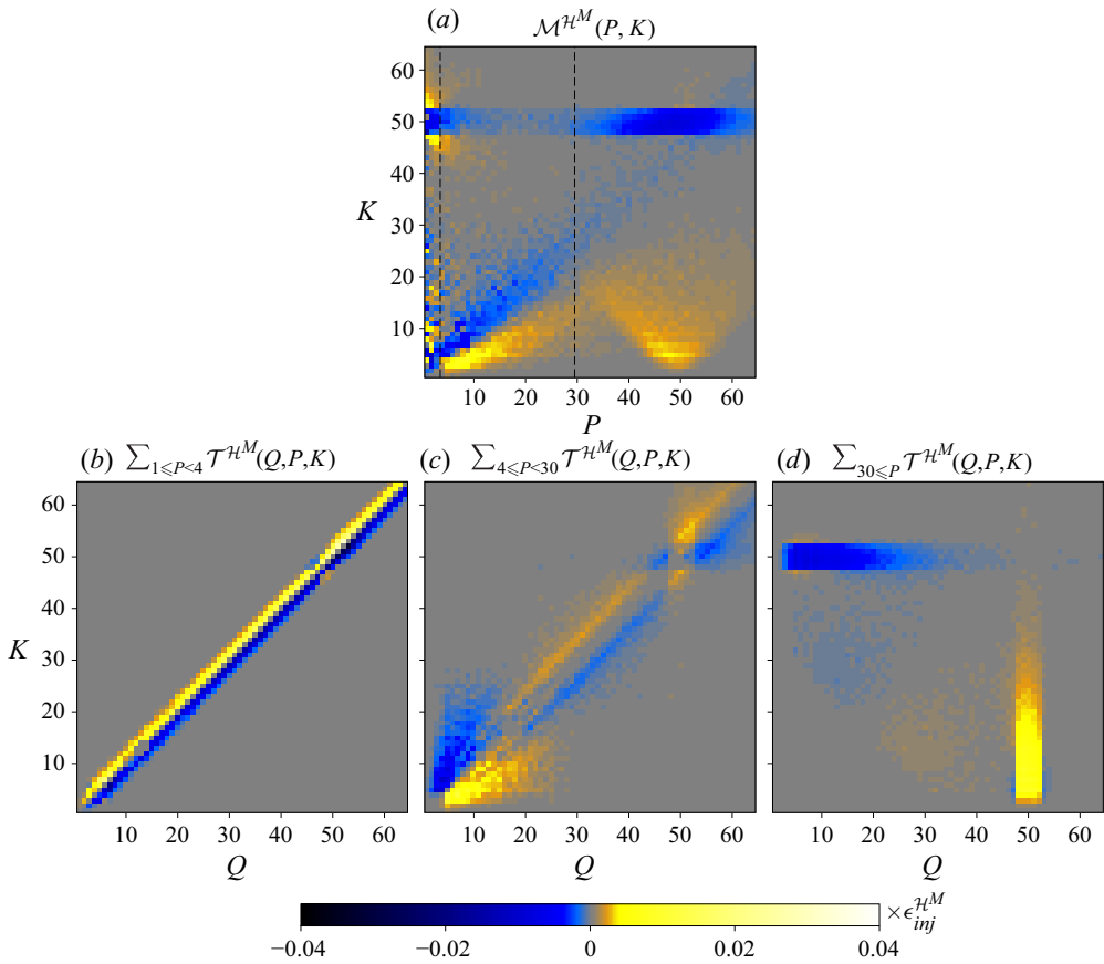
Figure 3. Role of the mediating velocity field, for run M8c at an instant when \mathcal{I}_{\mathcal{H}^M} \approx L/10 . (a) Sum of \mathcal{T}^{\mathcal{H}^M}(Q, P, K) along Q . (b–d) Sum of \mathcal{T}^{\mathcal{H}^M}(Q, P, K) along P for different velocity field shells, showing that the three features are associated with mediation at different scales.
