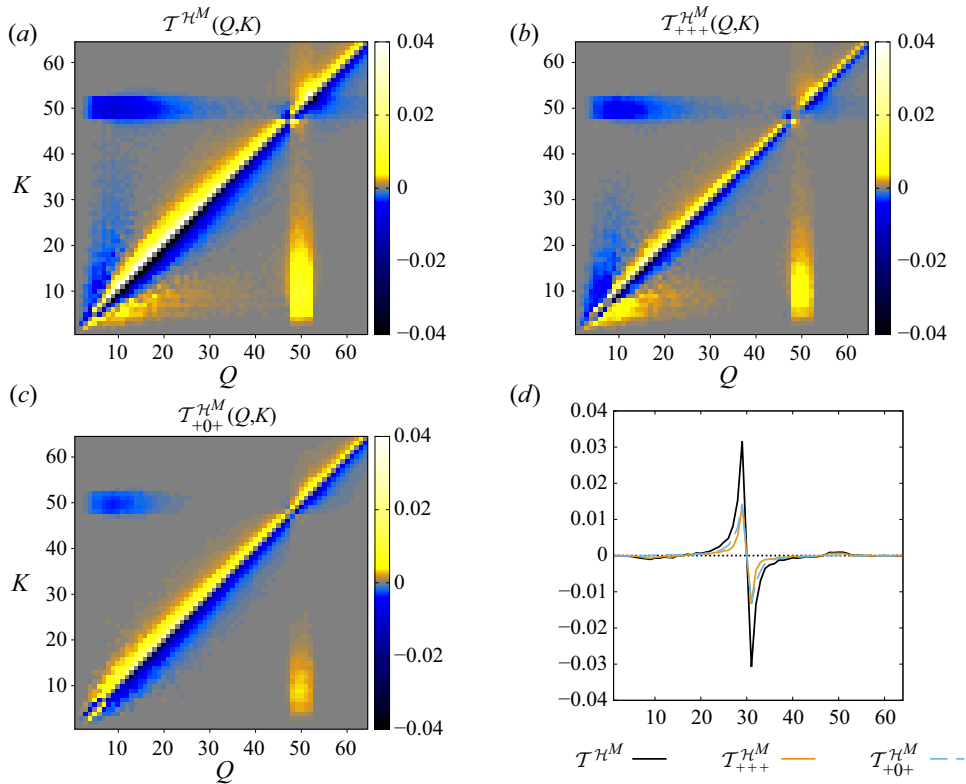
Figure 12. (a–c) Magnetic helicity transfer rates between the shells Q and K and their greatest helical contributions for the M11s run at an instant in time when \mathcal{I}_{\mathcal{H}^M} \approx L/10 . (d) Cuts of panels (a–c) at K_0 = 30 . The transfers are expressed in units of the magnetic helicity injection rate \epsilon_{inj}^{\mathcal{H}^M} .
