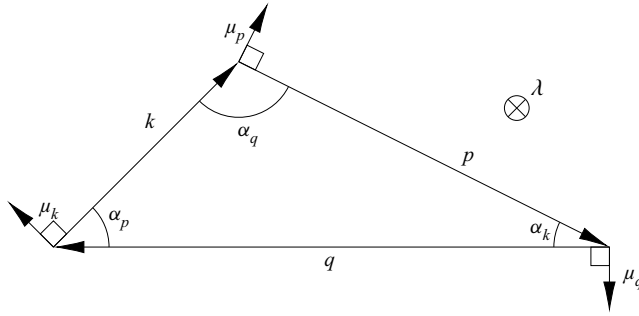
Figure 16. Definition of the notation for the derivations of the geometric triad factor. Redrawn from Waleffe (1992).
