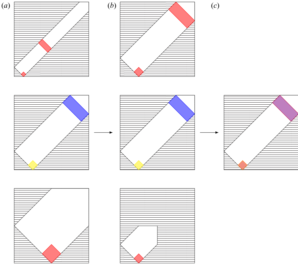
Figure 17. Illustration of the algorithm generating figure 10. (a) Three slices being merged. (b) After resizing so that their angles coincide. (c) The final merged picture. The sum of the red and blue bands from the top and middle pictures gives the purple band, which is normalised by a factor 2, since only two of the three slices contributed to it. The smaller orange square is normalised by a factor 3 since it comes from all three slices.
