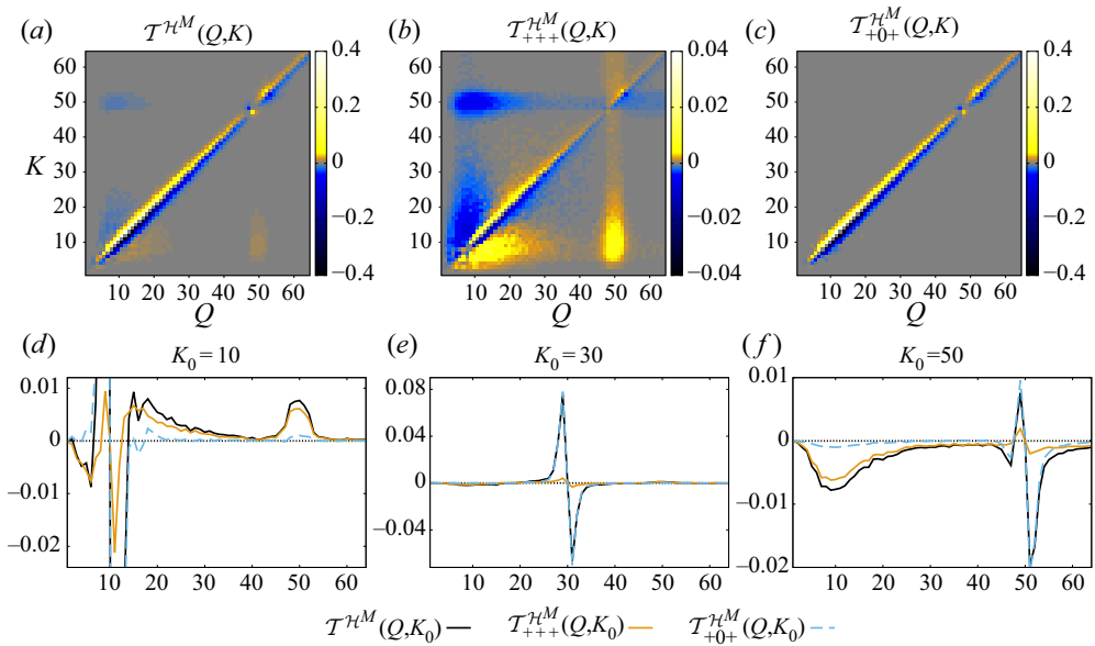
Figure 13. (a–c) Magnetic helicity transfer rates between the shells Q and K and their greatest helical contributions for the M1c run at an instant when \mathcal{I}_{\mathcal{H}^M} \approx L/10 . Please note that the extremes of the colour bar of panel (b) are an order of magnitude lower as compared to panels (a) and (c). (d–f) Cuts of panels (a–c) at K_0 = 10 , K_0 = 30 and K_0 = 50 , respectively. The transfers are expressed in units of the magnetic helicity injection rate \epsilon_{inj}^{\mathcal{H}^M} .
