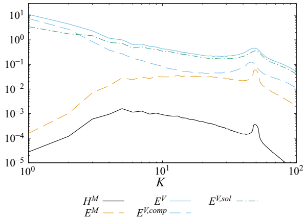
Figure 1. Magnetic helicity H^M , magnetic energy E^M and specific kinetic energy E^V spectra (decomposed into solenoidal E^{V,sol} = E^{V,+} + E^{V,-} and compressive E^{V,0} parts such that E^V = E^{V,sol} + E^{V,0} ) for the M8c run at an instant when \mathcal{I}_{\mathcal{H}^M} \approx L/10 .
