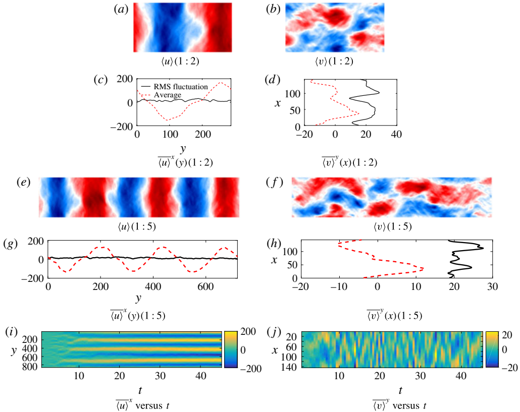
FIGURE 3. (a–h) Parallel and transverse barotropic velocity fields \langle u \rangle (a, c, e, g) and \langle v \rangle (b, d, f, h). Aspect ratios of 1:2 and 1:5 are depicted in (a, b, c, d) and (e, f, g, h) respectively. Here, \bar{f}^d indicates averaging of f in the d direction. The average and RMS fluctuations of \langle u \rangle in the parallel direction, i.e. averaging in the x direction, reveal a Kolmogorov-like velocity profile, and the fluctuations of \langle v \rangle in the transverse direction reveal the presence of a meandering jet (red dashed lines). The amplitude of the RMS fluctuations about these profiles is shown by solid black lines. (i, j) Hovmöller diagrams of (i) \langle u \rangle^x and (j) \langle v \rangle^y for an aspect ratio of 1:5 at time intervals \Delta t = 0.5 .
