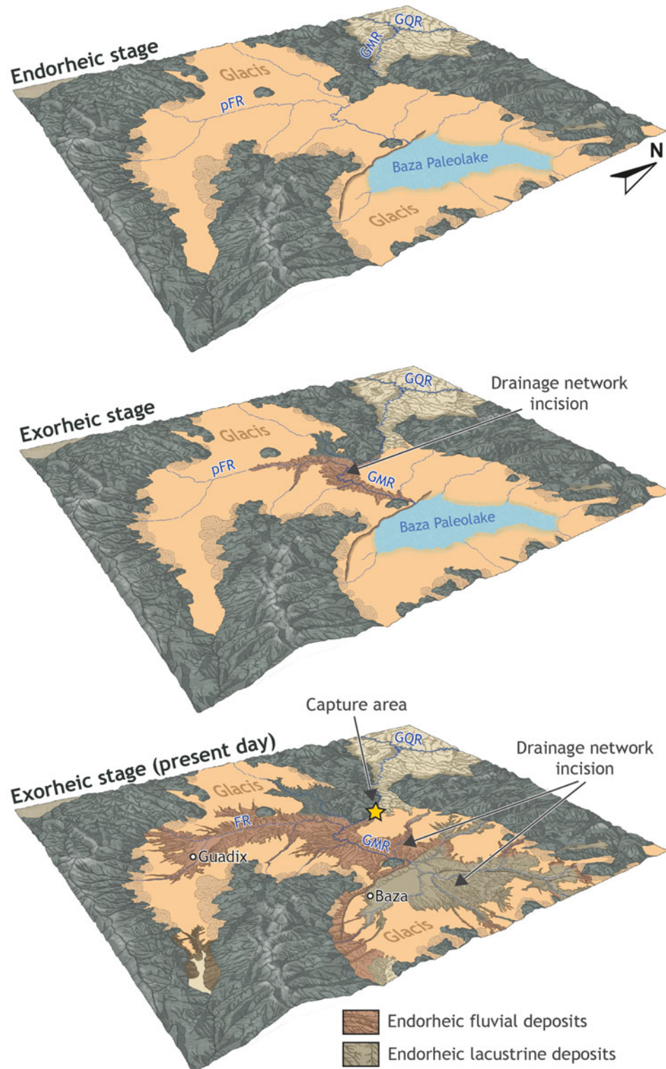
Figure 4. Sketches illustrating the Plio-Quaternary evolution of the Guadix-Baza Basin (GBB). During the initial endorheic stage, glacis developed throughout the entire basin. After the capture of the basin, the GBB became exorheic, and erosion has prevailed since that moment. pFR, Fardes paleo-River; FR, Fardes River; GQR, Guadalquivir River; GMR, Guadiana Menor River.
