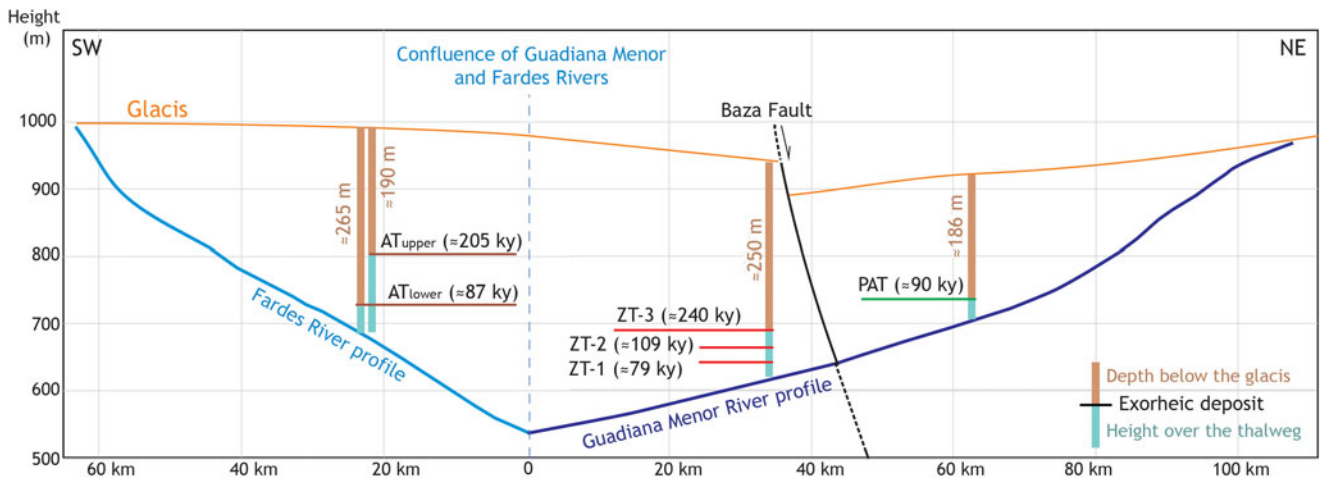
Figure 9. Numerical age and position of the exorheic deposits dated or included in the discussion of this study. They are depicted according to their depths below the glacia surface and the distances to the capture area, which is approximately the confluence between the Guadiana Menor and Fardes rivers (blue and purple longitudinal profiles). AT, Alicún travertines; ZT, Zújar travertines; PAT, Puente Arriba Terrace.
