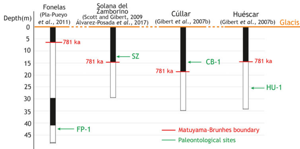
Figure 10. Sediment thickness between the glacia and the Matuyama-Brunhes reversal in different stratigraphic successions of the endorheic infilling of the Guadix-Baza Basin. The positions of the paleontological sites within these successions are indicated, along with the authors who identified the Matuyama-Brunhes reversal in each site (Gibert et al. , 2007b; Scott and Gibert, 2009; Pla-Pueyo et al. , 2011; Álvarez-Posada et al. , 2017).
