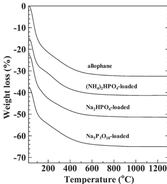
Figure 4. TG curves of allopahne and phosphate-loaded allopahnes.
