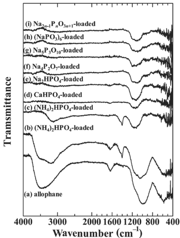
Figure 5. FTIR (a–b) and difference FTIR (c–i) spectra of allophane and phosphate-loaded allophanes.
