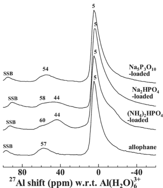
Figure 7. ^{27}\text{Al} MAS NMR spectra of allophane and phosphate-loaded allophanes. SSB: spinning side band.
