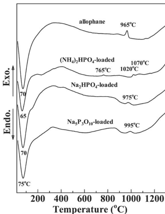
Figure 3. DTA curves of allopahne and phosphate-loaded allopahnes.
