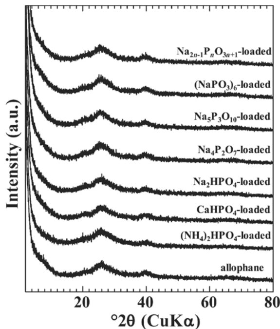
Figure 2. XRD patterns of allopahne and phosphate-loaded allopahnes.
