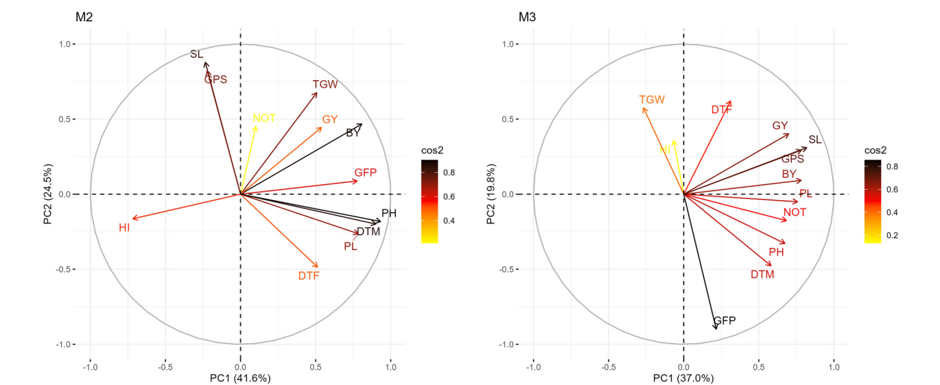
Figure 4. Quality of representation (cos2) of different traits in M 2 and M 3 generations of HPW 89; low cos2 values are coloured in 'yellow', mid cos2 values in 'red' and high cos2 values with 'black' colour.
