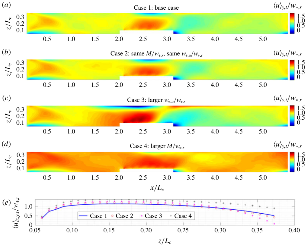
FIGURE 7. Pseudocolour plots of u (normalized by w_{*,r} ) for cases 1 (a), 2 (b), 3 (c) and 4 (d), and vertical profiles of u (normalized by w_{*,r} ) over the city for these cases (e).
