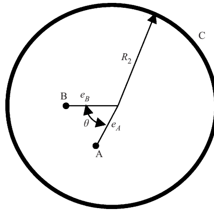
FIGURE 4. A schematic depiction of the location of the two inner electrodes A and B. e_A and e_B denote the distances of the electrodes from the cavity centre, and \theta is the angle between the radii that go through the electrode locations.
