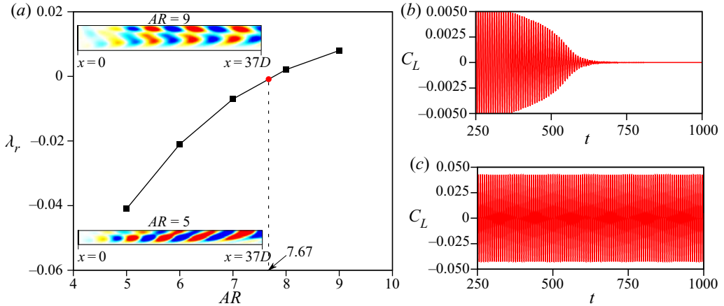
Figure 17. Flow past a cylinder with side wall at Re = 90 . (a) Variation of growth rate of the dominant mode with AR . The spanwise vorticity field in the x-z plane for the real part of the eigenmode corresponding to the eigenvalue with largest real part is shown in the inset for two values of AR . (b,c) Time histories of lift coefficient for the direct numerical simulations initiated with unsteady two-dimensional flow for (b) AR = 7 and (c) AR = 9 .
