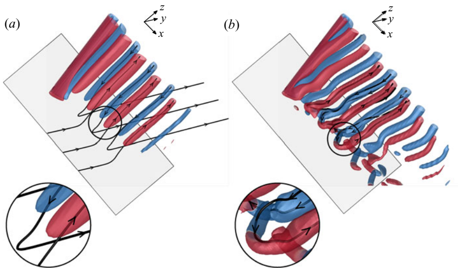
Figure 7. Flow past a cylinder with side wall: Q ( =0.002 ) iso-surfaces coloured with spanwise component of vorticity ( \omega_z = \pm 0.01 ) for the instantaneous flow depicting (a) diffused end vortex structures for (AR, Re) = (60, 50) at t = 1350 and (b) linked end vortex structures for (AR, Re) = (60, 75) at t = 1725 . Also shown are a few vortex lines for each case that pass through the core of the vortices at the plane of symmetry and the enlarged view of the images next to the side wall. The side wall ( z = 0 ) is shown for reference.
