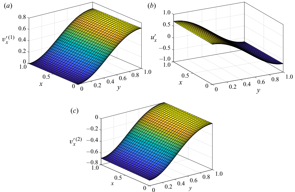
FIGURE 3. The normalised perturbations, for the fluids and DS, at a = 0.6 , b = 1 , \Gamma = 0.57 , \mu_r = 0.5 , k = 0.029 , \Sigma_1 = 1 , \Sigma_2 = 1 and V_r = 0 for the marginally stable eigenvalue \omega = 0.01001 . Here, v'_x(1) = \text{Re}[\tilde{v}_x^{(1)} e^{ikx}] , v'_x(2) = \text{Re}[\tilde{v}_x^{(2)} e^{ikx}] and u'_x = \text{Re}[\tilde{u}_x e^{ikx}] . For convenience, the axes for the fluids and DS have been normalised to the interval [0, 1] . The length of the domain in the x -direction is equal to a wavelength ( 2\pi/k ) of the perturbations. The plots show that the unstable eigenmode is antisymmetric. (a) v'_x(1) ; (b) u'_x ; and (c) v'_x(2) .
