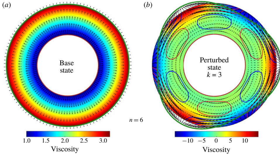
FIGURE 3. (Colour online) The base state and a perturbed state for n = 6 , R_0 = 2 . (a) The base state is axisymmetric with radially growing viscosity \mu_0 (colour). (b) The perturbation flow for k = 3 , showing the perturbation viscosity (colour), velocity field (arrows) and streamlines (blue and red curves), where \mathcal{G} = 0.1 . In both panels (—, brown) marks the inner boundary r_G , and (—, green) marks the leading front r_N .
