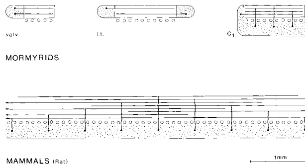
Figure 2 (Meek). Schematic transverse views of cerebellar configurations in mormyrids and mammals. Stipples and dots are granule cells, open circles are Purkinje cell bodies, and horizontal lines are parallel fibers. Valv. = valvula cerebelli; l.t. = lobus transitorius cerebelli; and C 1 = cerebellar lobe C 1 .
