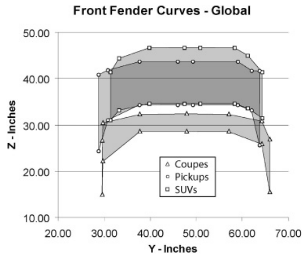
Fig. 30. The front fender curve global coordinate system. The grey area surrounded by a symbol shows the allowable range for the control points to stay within the designated vehicle class.
