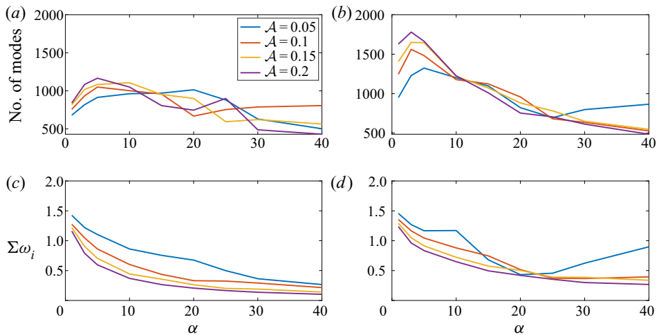
Figure 11. The number of unstable modes (a,b) and the sum of positive growth rates (c,d) as functions of \alpha : (a,c) in the presence of ZR; (b,d) in the presence of MR.
