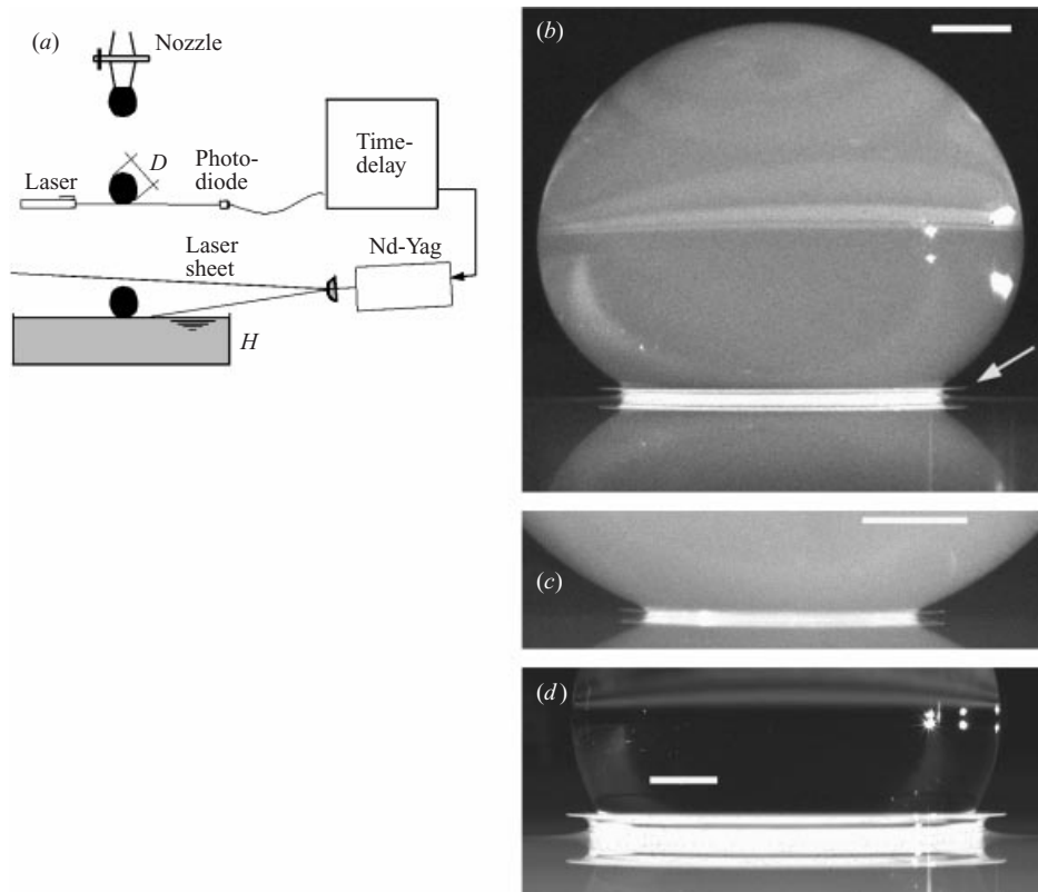
FIGURE 1. Examples of ejecta sheets. (a) Sketch showing the experimental setup. The ejecta sheets are shown for the following impact conditions: (b) \mu = 43 cP, U = 6.2 m s -1 ( Re = 1080 , We = 4170 ), (c) \mu = 7.1 cP, U = 4.65 m s -1 ( Re = 4640 , We = 2190 ), (d) \mu = 73 cP, U = 4.65 m s -1 ( Re = 480 , We = 2370 ). The arrow points to the sheet. The lower images in each panel are reflections in the free surface. The scale bars are 1 mm long. The drop liquid in the bottom panel has not been dyed with Fluorescein.
