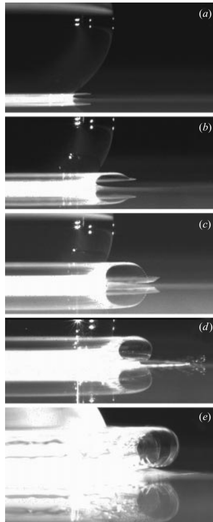
FIGURE 5. Evolution of the ejecta sheet for low viscosity, showing the typical bending of the sheet and impact with the bottom layer, sending off tiny droplets; \mu = 16 cP, U = 4.65 m s -1 and D = 6.5 mm. The instants shown are (a) 80 \mu s, (b) 150 \mu s, (c) 190 \mu s, (d) 270 \mu s and (e) 480 \mu s after the initial contact.
