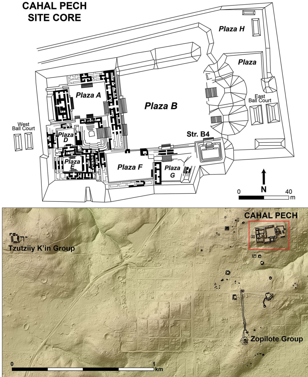
Figure 3. Cahal Pech centre (top) and peripheral settlements examined in this study (bottom; maps by C. Ebert).
