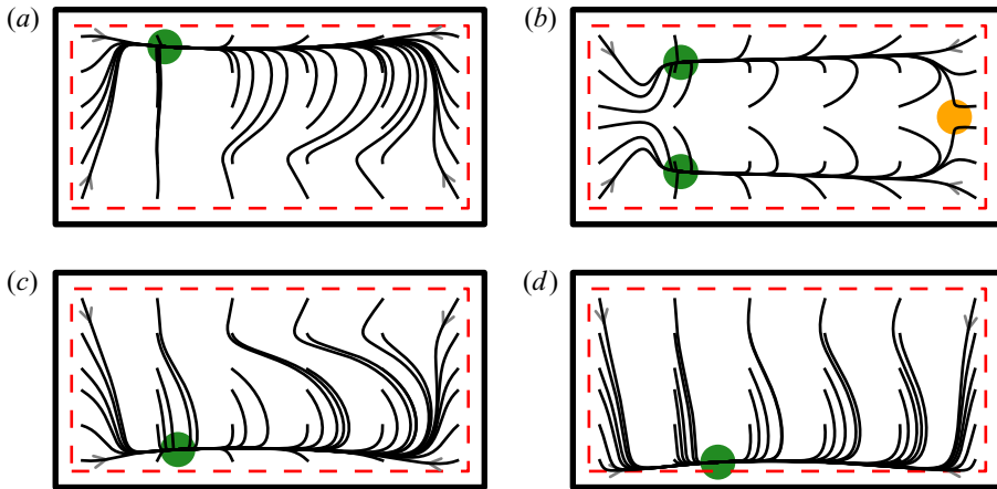
FIGURE 10. Estimated particle trajectories for \rho_s = -1, 0, 1, 3 (a,b,c,d) with 2R/\ell = 160 and Fr^2 = 1 for a particle with radius 2a/\ell = 0.15 . Green and yellow markers show the stable and saddle equilibria, respectively, with size matching that of the particle.
