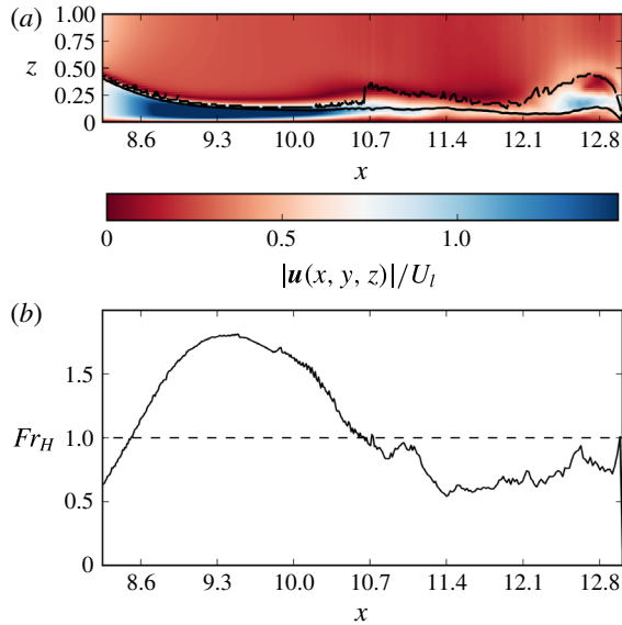
FIGURE 9. (a) Non-dimensional velocity |\mathbf{u}|/U_l on the mid-plane y=y_0 ; the thick black line indicates the depth h_l = \overline{g'h}/g' and the dashed line marks h_i , i.e. the interface \rho = 3\% , (b) Froude number Fr_H versus x . Case S3, t = 16 .
