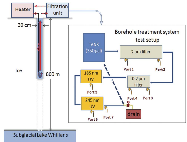
Fig. 2. Schematic (left panel, not to scale) showing the flow directions for the field operation of the Whillans Ice Stream Subglacial Access Research Drilling (WISSARD) water treatment system. The filtration and UV-treatment unit will be placed in-line between the borehole water return line and the heater modules. The enlarged inset (right panel) shows the treatment system components as set up for the laboratory tests. See text for details.
