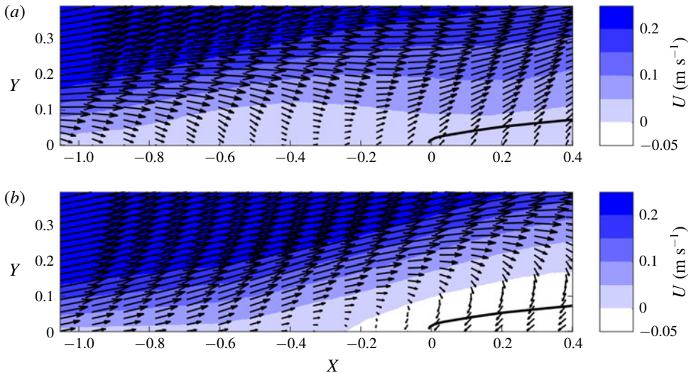
FIGURE 15. (Colour online) A ROM reconstructed using the mean flow and the second POD mode ( \langle U \rangle + a_2^2 \phi^2 ). Two instants with (a) a_2^2 = 10 and (b) a_2^2 = -10 are selected. The solid lines show contours of \langle U \rangle = 0 .
