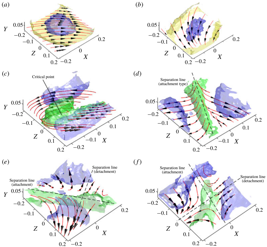
FIGURE 16. (Colour online) 3D spatial organization of POD modes obtained from tomo-PIV showing the (a) first, (b) second, (c) third, (d) fourth, (e) fifth and (f) sixth most energetic modes. The dark grey (blue online), bright grey (yellow online) and medium grey (green online) contours represent isosurfaces of normalized magnitude of the mode magnitude at |\phi^i| = 0.0033 , 0.0025 and 0.0012 , respectively. The streamlines visualize the 3D spatial pattern of the modes.
