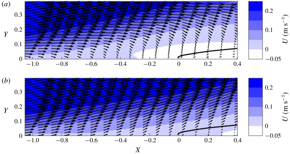
FIGURE 14. (Colour online) A ROM reconstructed using the mean flow and the first POD mode ( \langle U \rangle + a_1^1 \phi^1 ). Two instants with (a) a_1^1 = 10 and (b) a_1^1 = -10 are selected. The solid lines show contours of \langle U \rangle = 0 from the mean velocity profile of figure 4(a).
