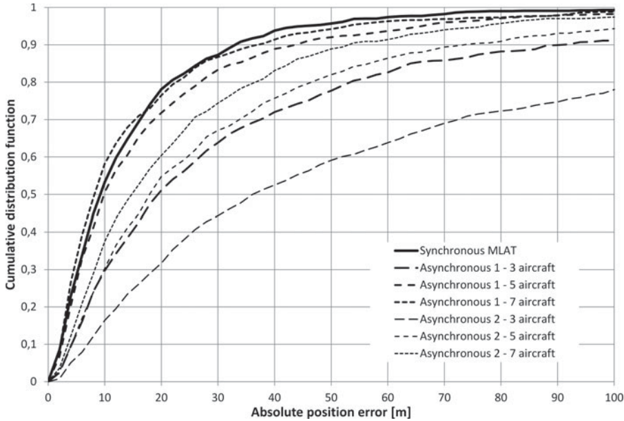
Figure 3. Cumulative distribution of the absolute position error for synchronous and asynchronous MLAT with time measurement errors modelled by a normal distribution with a standard deviation 3\text{ns} .
