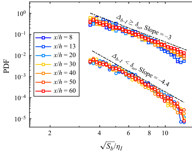
Figure 14. The PDFs of the bubble size at different streamwise positions. The bubble size is characterized by the square root of the bubble area S_b . The PDFs for \Delta_{b-1} < \delta_\omega are offset by 10^{-2} for clarity.
