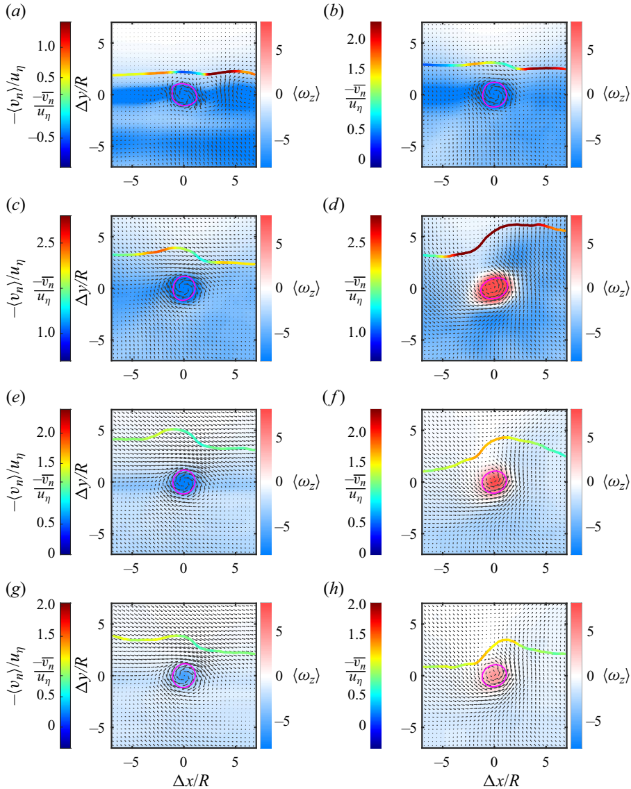
Figure 16. Conditional averaged flow fields in the vicinity of vortex structures. The conditional fluctuation velocity vectors are superimposed on the contour map of conditional averaged vorticity \langle \omega_z \rangle . The vortex structure boundary is indicated by the magenta contour of the conditional averaged swirling strength \langle \lambda_{ci} \rangle = 0.2 \langle \lambda_{ci} \rangle_{max} . The conditional averaged position of the TNTI is presented by the jet-coloured open curve, whose colour represents the magnitude of conditioned averaged entrainment velocity \langle v_n \rangle . The colour bar of \langle v_n \rangle (left) is centred at the ensemble averaged entrainment velocity \bar{v}_n to make it convenient to identify the increase or decrease in the entrainment velocity through colour. Data for conditional analysis are obtained in the vicinity of (a,b,c,e,g) prograde and (d,f,h) retrograde vortex structures at (a) x = 7.5h , (b) x = 10h , (c,d) x = 13h , (e,f) x = 30h and (h,g) x = 55h , respectively.
