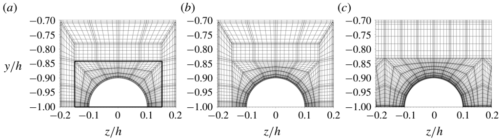
FIGURE 28. Mesh refinement around the hemispherical roughness for the rough-wall case at Re_\tau = 300 with k/h = 0.1 and d/k = 4 . (a) Coarse (M3), 67, 584 grid points/cell; (b) moderate (M2), 215, 040 grid points/cell; (c) fine (M1), 387, 072 grid points/cell. Box in (a) denotes the boundary of the refined region (cell) enclosing each hemisphere.
