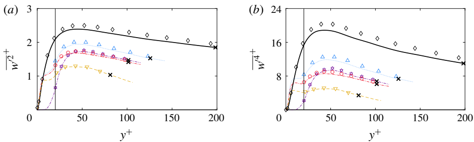
FIGURE 21. (Colour online) Predictions of (a) \overline{w'^2}^+ and (b) \overline{w'^4}^+ for the smooth- and rough-wall cases in comparison with the original DNS statistics. Symbol \times marks the reference location where the large-scale signal is extracted. Vertical line denotes the location of the roughness crest k^+ = 20 . Legend as in figure 13.
