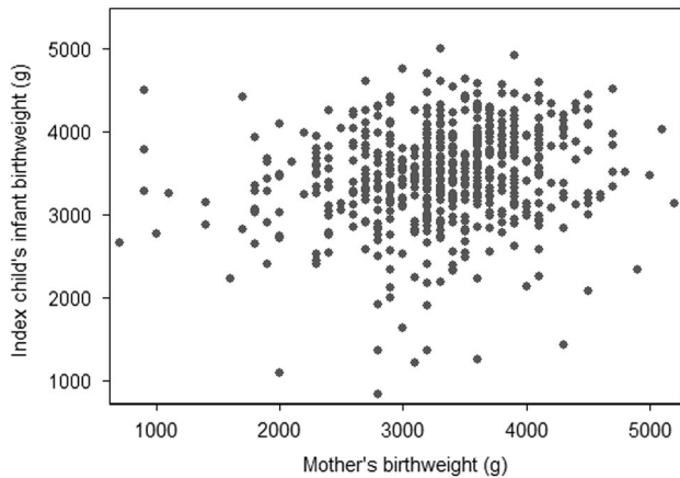
Fig. 1. Correlation between mother's birth weight and index child's infants birth weight in the Lifeways Cross-Generation Cohort Study ( n = 613 ).
