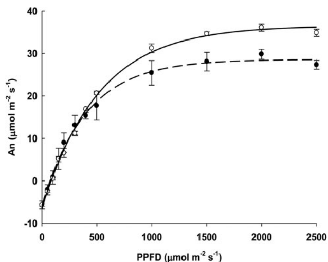
Fig. 2. Net CO 2 assimilation rate ( A n ) as a function of the photosynthetic photon flux density (PPFD). (○, —) Low density; (●, ----) high density. Each point is the mean ± SD of five independent measurements. Vertical bars indicate SD.
