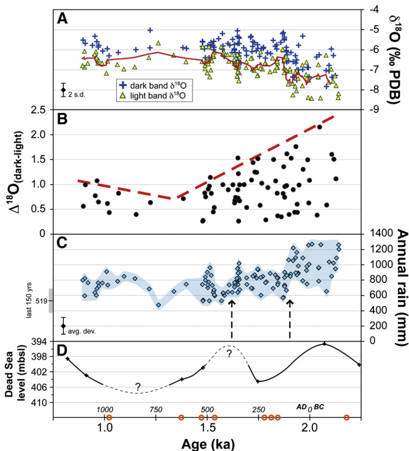
Figure 6. Panel A shows the measured \delta^{18}\text{O} (PDB) values for ion microprobe analysis of light and dark fluorescent calcite bands across Soreq Cave sample 2–6. Analytical precision (2 s.d. = \pm 0.34\% ) is illustrated in the lower left of panel A. For all 75 bands analyzed in this sample, the dark fluorescent calcite always has a higher \delta^{18}\text{O} value than its coupled light fluorescent calcite. In general, for light fluorescent calcite, higher \delta^{18}\text{O} values represent drier climates while lower \delta^{18}\text{O} values are characteristic of wetter climates (see text for explanation). The heavy line, a 6-point running average, shows the general variability of \delta^{18}\text{O}_{\text{light calcite}} values from 2.2–0.9 ka. Panel B shows values of \Delta^{18}\text{O}_{\text{dark-light}} ( \delta^{18}\text{O}_{\text{dark calcite}} - \delta^{18}\text{O}_{\text{light calcite}} ) of individual annual bands. The heavy dashed line emphasizes the decrease in maximum \Delta^{18}\text{O}_{\text{dark-light}} values from 2.0–1.3 ka. Panel C plots estimates of annual precipitation amounts (mm) calculated from the \delta^{18}\text{O} values of wet-season calcite (light fluorescence) assuming a dripwater temperature of 19^\circ\text{C} and Eq. (1); the dashed arrows highlight sharp decreases in annual rainfall amounts at \sim 1.9 and 1.6 ka. The shaded region represents the range of rainfall estimates calculated for dripwater temperature between 18 and 20^\circ\text{C} . The average deviation of modern rainfall data from Eq. (1) is shown in the lower left of panel C. The mean and 1 s.d. range of annual rainfall in Jerusalem for the last 150 yr, as collected by the Israel Meteorological Survey, is plotted on the left axis. Panel D illustrates concurrent changes in another paleorainfall proxy for the Levant region, the Dead Sea level (mbsl; Bookman et al., 2004). The circles along the age-axis represent the eight U-series dates (ka) acquired by MC-ICP-MS (Table 1).
