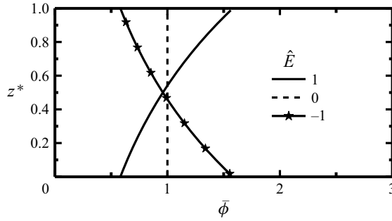
Figure 2. Basic-state solutions of \bar{\phi} for three typical values of \hat{E} .
