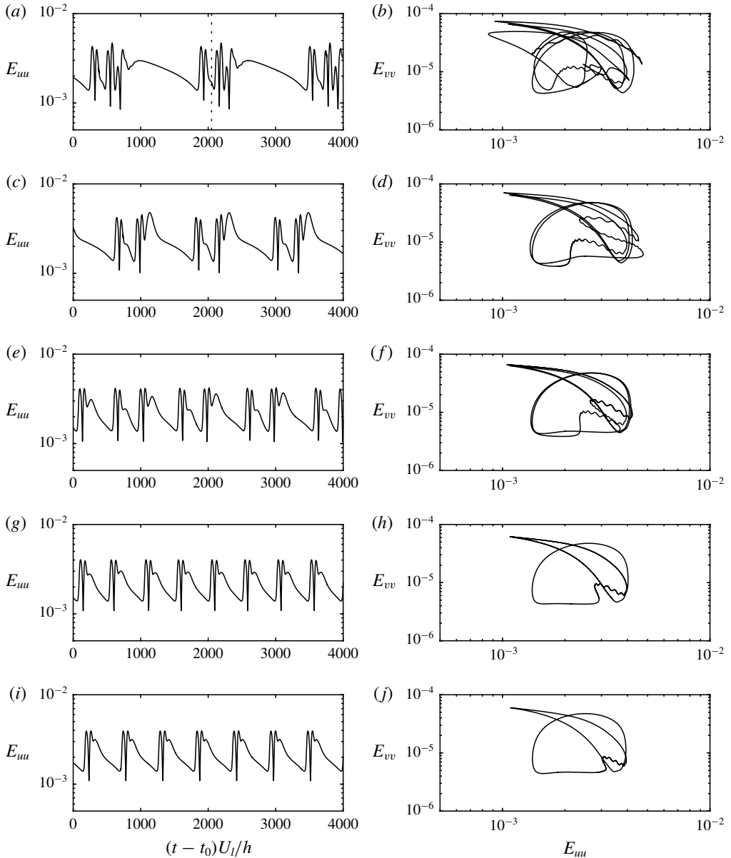
FIGURE 5. Periodic orbits of the edge state for Poiseuille flow for various control amplitudes: (a,c,e,g,i) E_{uu} against (t - t_0)U_l/h , where t_0 is the time of the initial velocity field; (b,d,f,h,j) E_{uu} versus E_{vv} . (a,c,e,g,i) correspond to \phi = 0.0, 0.1, 0.2, 0.5, 1.0 , respectively; likewise for (b,d,f,h,j).
