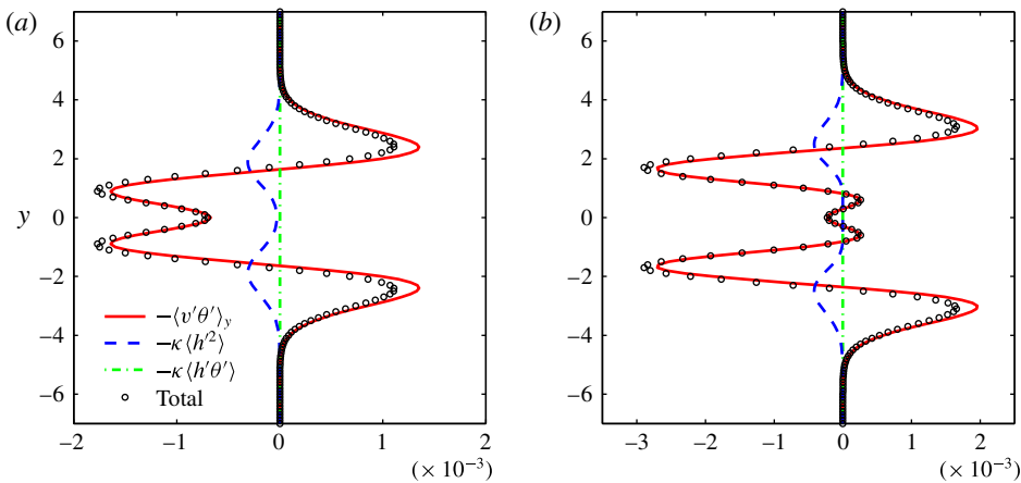
FIGURE 15. (Colour online) The effective thermal terms -\langle v'\theta' \rangle_y , -\kappa \langle h^2 \rangle , -\kappa \langle h'\theta' \rangle on the right-hand side of (5.20), and their sum, for dissipation solely by radiative relaxation ( \kappa = 0.002 , \gamma = 0 ). All terms are calculated for k = 1 , a = 1 for scaling, and either (a) n = 1 or (b) n = 2 .
