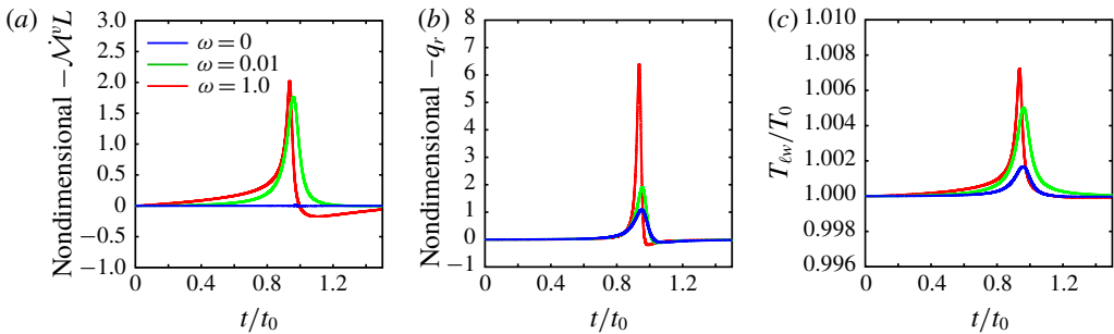
FIGURE 5. (Colour online) Time evolution of (a) the energy flux due to latent heat of condensation/evaporation -\dot{\mathcal{M}}^v L , (b) heat flux -q_r , and (c) liquid temperature T_{\ell w} when the first bubble collapse in the case of R_0 = 50 \times \ell_0^v , N_0 = 1.0 and p_{\ell\infty}/p_0 = 5.0 .
