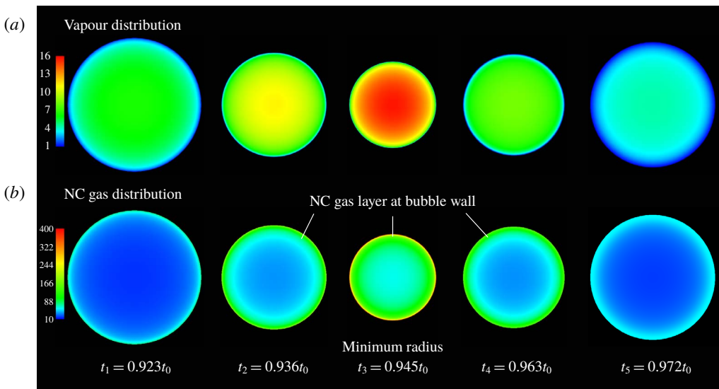
FIGURE 6. (Colour online) Snapshots of the density distribution of vapour and NC gas inside the bubble when \omega = 1.0 , R_0 = 50 \times \ell_0^v , N_0 = 1.0 and p_{\ell\infty}/p_0 = 5.0 : (a) vapour and (b) NC gas, where t_1 = 0.923 t_0 , t_2 = 0.936 t_0 , t_3 = 0.945 t_0 , t_4 = 0.963 t_0 and t_5 = 0.972 t_0 .
