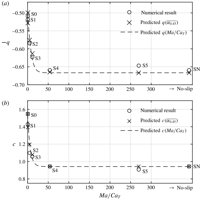
FIGURE 15. Variation of (a) exponent -q and (b) constant c with Ma/Ca_T . Note results are averaged from t = 150-300 and the least-squares method was used to extract -q and c from the numerical results.
