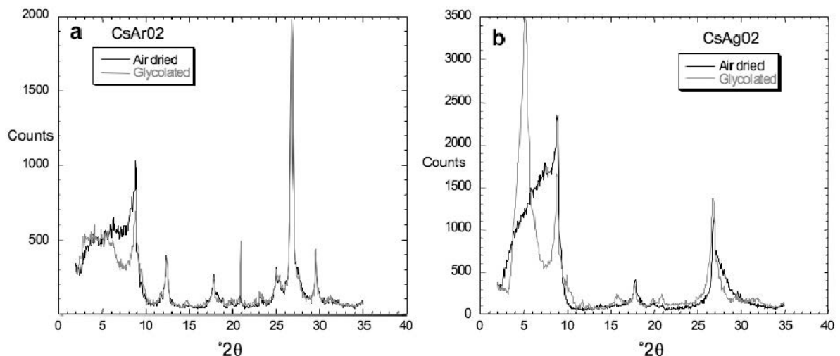
Figure 4. Oriented clay mount XRD patterns ( \text{CuK}\alpha radiation) of <2.0 \mu\text{m} clay fractions of the (a) CsAr02 and (b) CsAg02 clays. Comparison of the air-dried to ethylene glycol vapor-treated preparations indicates the abundance of expandable clay (smectite).
