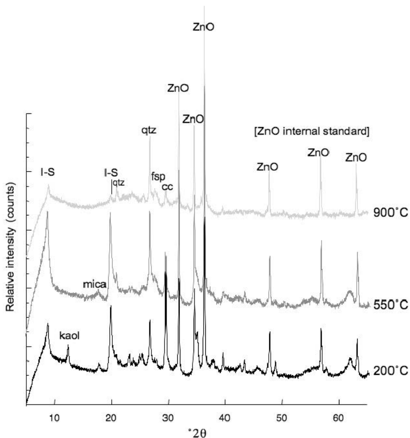
Figure 5. Random powder XRD patterns (CuK \alpha radiation) of heated CsAg02 clay showing loss of smectite as the clay structure breaks down.
