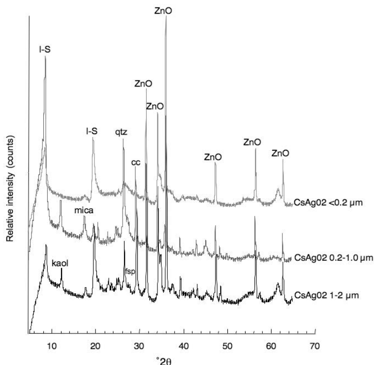
Figure 3. Random powder XRD patterns (CuK \alpha radiation) of different size fractions of the antibacterial CsAg02 clay, showing more detrital minerals in the coarser fractions, e.g. quartz (qtz), feldspar (fsp), calcite (cc), kaolinite (kaol).
