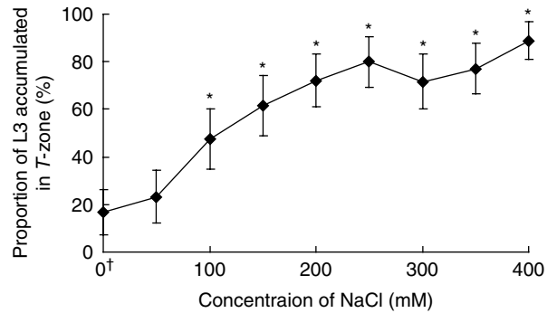
Fig. 3. The effect of NaCl concentration on the chemotactic responses of infective third-stage larvae (L3) of Brugia pahangi . Each error bar shows the 95% confidence interval for the proportion of L3 accumulating in the T-zone. * P < 0.01 , the proportion of L3 accumulating in the T-zone of NaCl at different concentrations was compared with that of deionized water (DW), z-test. †Control (DW alone in the T-zone).
