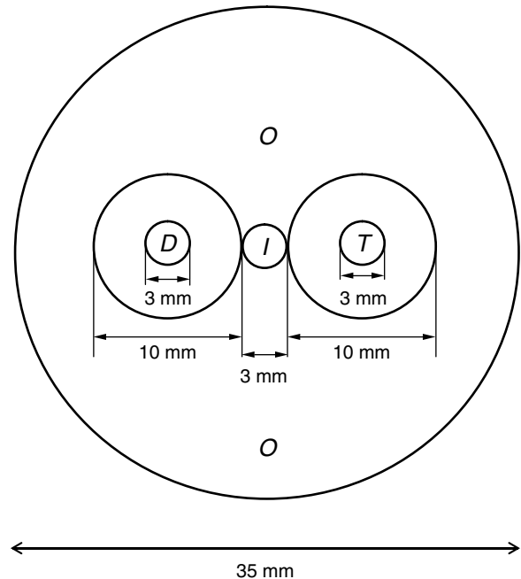
Fig. 1. Diagrammatic representation of the sectors used to quantify the larval response to test solutions. The small circles marked by I , D and T , indicate the areas on to which 1 \mu l of deionized water (DW) and infective third-stage larvae ( I -area), 2 \mu l of DW alone ( D -area) and test solution ( T -area) were placed, respectively. The large concentric circles were marked as D - and T -zones, and the outside zone was marked as O .
