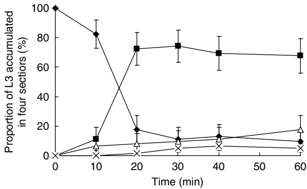
Fig. 2. The time course of the chemotactic response of infective third-stage larvae (L3) of Brugia pahangi to fetal bovine serum (FBS). Four sectors are indicated as follows: ◆, I-area; ■, FBS-zone; △, O-zone; ×, D-zone. Each error bar shows the 95% confidence interval for the proportion of L3 accumulating in each sector.
