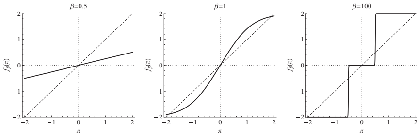
FIGURE 2. Low-information costs case. The map f_\beta in the system with three belief types for different values of \beta . The parameter values are b = 1 , C = 0 , and \phi_\pi = 0.5 .
