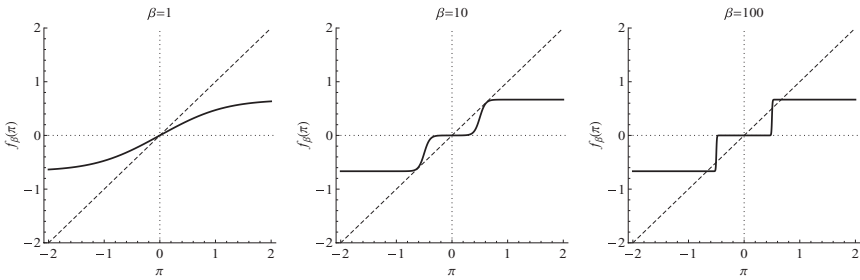
FIGURE 3. Low-information costs case. The map f_\beta in the system with three belief types for different values of \beta . The parameter values are b = 1 , C = 0 , and \phi_\pi = 1.5 .
