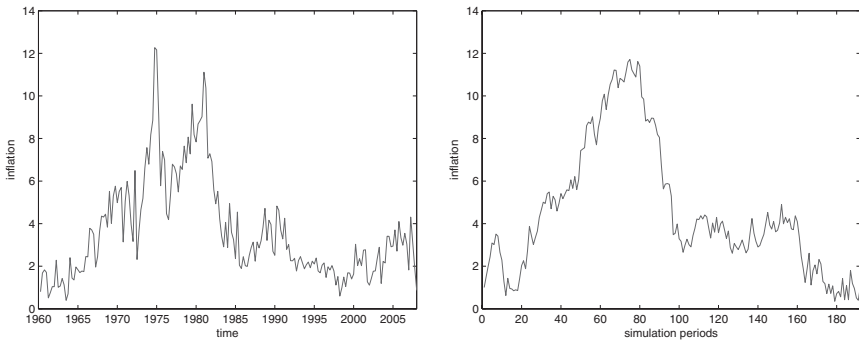
FIGURE 1. Inflation time series. Left: U.S. annualized inflation: quarterly data for the period 1960–2007. Right: Simulated data.
