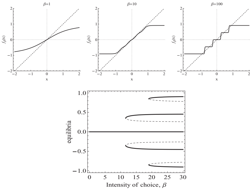
FIGURE 6. Top panels: The map f_\beta in the system with five belief types, b_h \in \{-1, -1/2, 0, 1/2, 1\} , for different values of \beta . The parameter values are b = 1, C = 0 , and \phi_\pi = 1.1 . Bottom panel: Bifurcation diagram for this system with the same parameter values with respect to the intensity of choice. Solid lines indicate stable equilibria and dashed lines unstable equilibria. For high values of \beta , nine different steady states co-exist, five stable separated by four unstable steady states.
