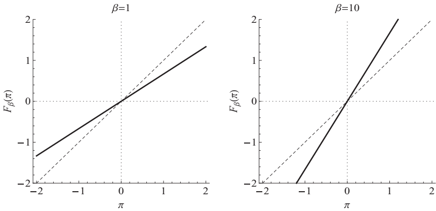
FIGURE 7. Graphs of the LTL map F_\beta in (11) when the Taylor principle is not satisfied for a normal distribution \psi(b) \simeq N(0, 0.25) of initial beliefs. The reaction coefficient is \phi_\pi = 0.5 . Left: \beta = 1 . Right: \beta = 10 .
