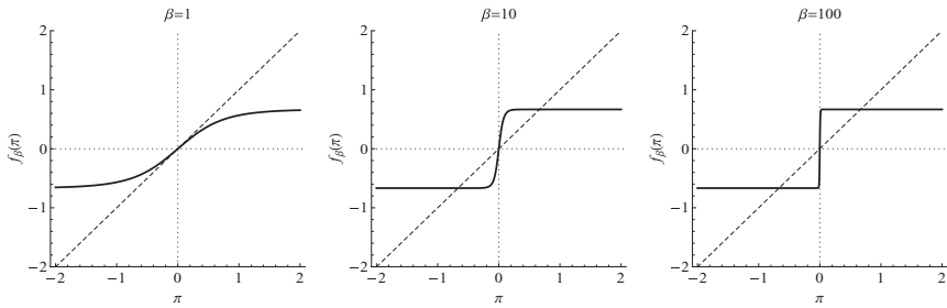
FIGURE 5. High-information costs case. The map f_\beta in the system with three belief types for different values of \beta . The parameter values are b = 1 , C = 1 , and \phi_\pi = 1.5 .
