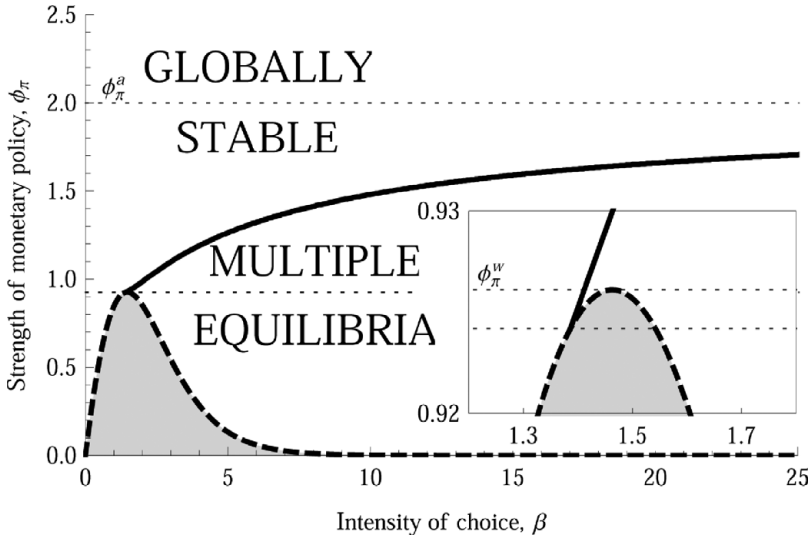
FIGURE B.1. Bifurcation diagram of dynamics in the low-cost case, shown in coordinates (\beta, \phi_\pi) . Parameters are C = 0 and b = 1 . The dashed curve gives all the parameters of the pitchfork bifurcation, whereas the solid line gives the parameters of the tangent bifurcation. The inset zooms the area where the curve of pitchfork bifurcation (dashed) intersects the curve of tangent bifurcation (solid). The shaded area represents the region in the parameter space in which the RE is locally unstable.
