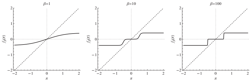
FIGURE 4. Low-information costs case. The map f_\beta in the system with three belief types for different values of \beta . The parameter values are b = 1 , C = 0 , and \phi_\pi = 2.5 .
