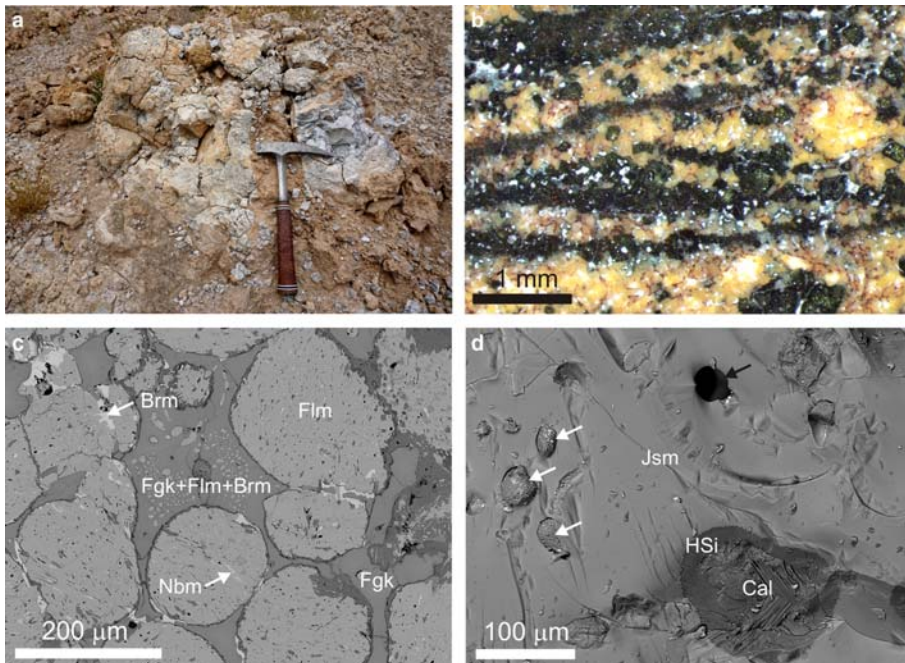
FIG. 3. (a) Jasmundite rock outcrop on the south slope of the Jabel Harmun, where dzierżanowskite was found. (b) Dark-green jasmundite crystals form chain-like aggregates along fissures in altered flamite rock; brownmillerite rims (red) are visible on flamite grains (yellow). (c) Altered flamite rock: BSE image of a yellow fragment of the rock. (d) Fresh fracture of a jasmundite crystal; oval inclusions of flamite relics are shown by white arrows; and a hollow channel is shown by a black arrow. A channel with hydrated walls filled by calcite is visible at bottom right corner. DZR = dzierżanowskite, Flm = flamite, Brm = brownmillerite, Nbm = nabimusaita, Fgk = fluorokuygenite, Cal = calcite, Jsm = jasmundite, HSi = hydrosilicate.
