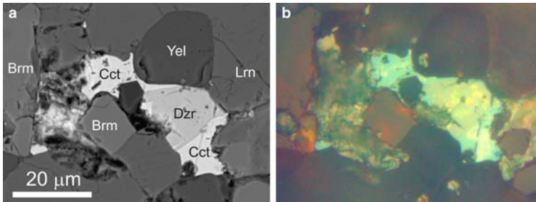
FIG. 2. One of the largest segregations of dzierżanowskite in holotype specimen MII-33: (a) BSE image. (b) Reflected light, poor polishing of chalcocite has resulted in its blue hue (covellite); dzierżanowskite is grey with cream hue, light-orange internal reflexes are visible in it; brownmillerite shows red internal reflexes. DZR = dzierżanowskite, Cct = chalcocite, Lrn = lamite, Brm = brownmillerite, Yel = ye'elimite.
