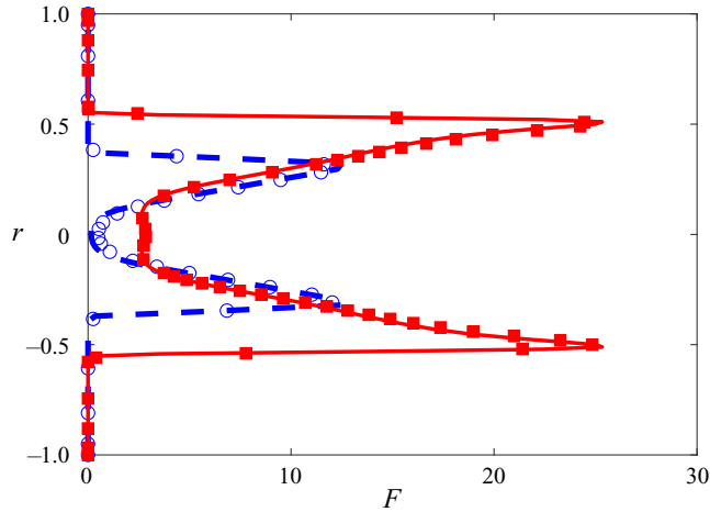
FIGURE 1. This figure shows a comparison of the numerically calculated baffle profile F at \alpha = 1.005 (lines) and the prediction from (4.3) (symbols). Two different values, a = 1 (blue-dashed line) and a = 4 (red-solid line), are shown. The good agreement confirms the assumption made in (4.2).
