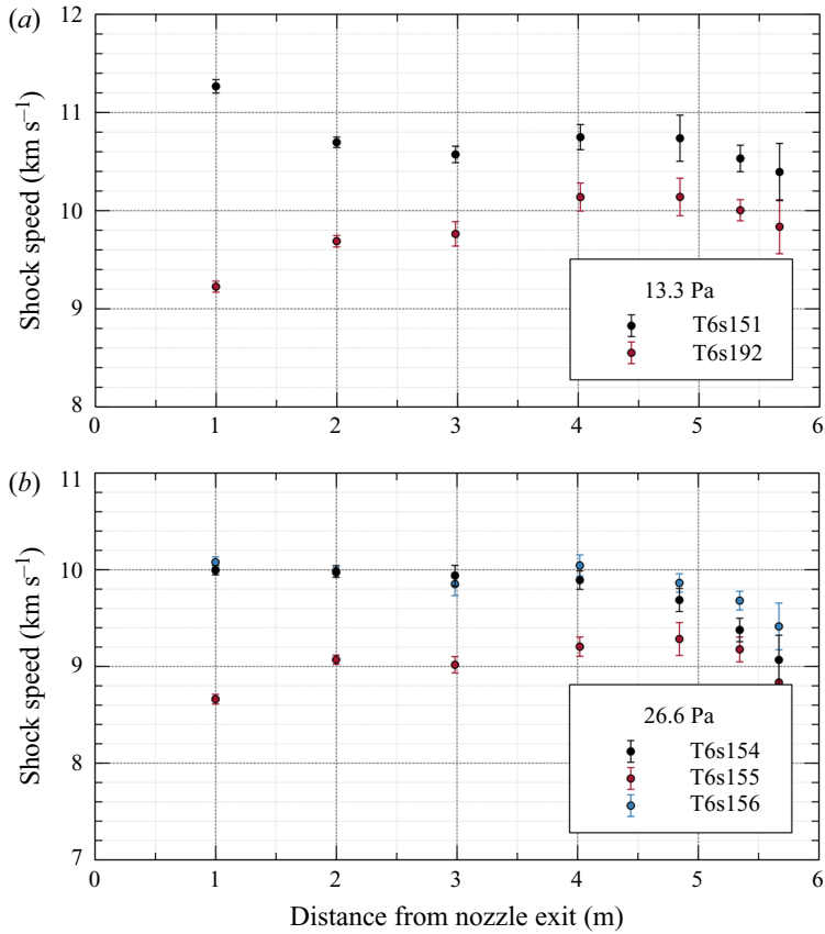
Figure 12. Measured SSV for the T6 electron density measurements.
