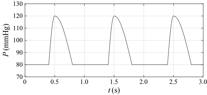
Figure 3. Model of pressure pulses released from a ventricle for T_0 = 0 s, T_1 = 0.1 s, T_2 = 0.3 s.
