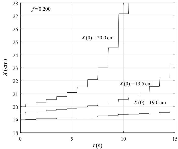
Figure 10. Balloon displacement for f = 0.200 and different X(0) . Other inputs are the same as those in figure 7.
