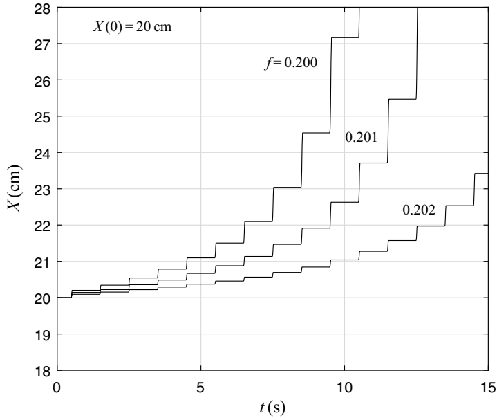
Figure 9. Balloon displacement for X(0) = 20 cm and different f . Other inputs are the same as those in figure 7.
