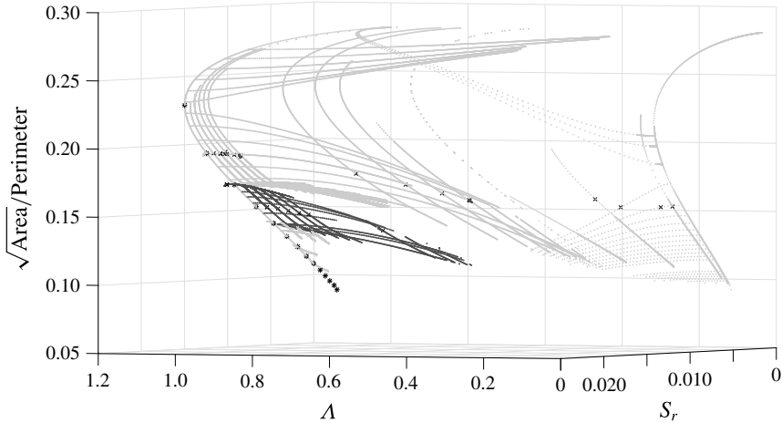
FIGURE 16. The family of Sadovskii solutions connecting the doubly cusped solutions at the m=4 patch bifurcation with the solutions with two pinch-off points at the m=6 patch bifurcation is shown in the darker color. All other Sadovskii solutions are shown in lighter grey.
