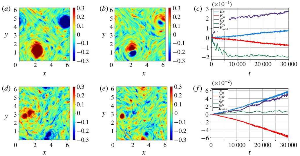
FIGURE 9. (Colour online) Top row shows the spatial structure of (a) \zeta_T and (b) q_C , both at t = 30\,000 , and (c) energy transfer time series for the SW_a case. (d–f) Shows the same quantities for the SW_b case.
