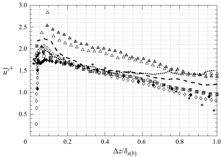
Figure 7. Streamwise velocity fluctuations \overline{u'^+} = \sqrt{u'^2}/u_\tau^* modified by different coverages. Symbols as in figure 5 and 6.
