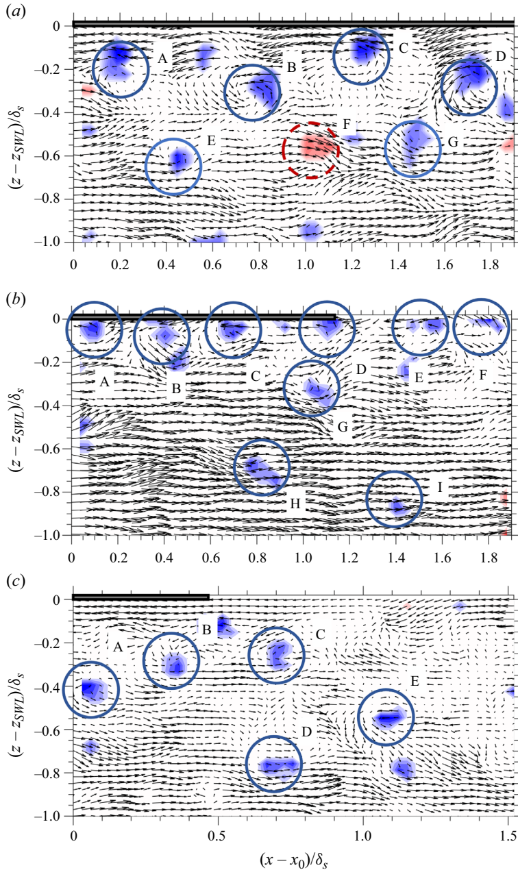
Figure 12. Examples of prograde and retrograde spanwise vortices via Galilean decomposition of instantaneous velocity fields in the streamwise–wall-normal plane of (a) 100 % coverage, (b) 60 % coverage and (c) 30 % coverage. Here U_c \approx 0.6U_{max} . The blue colour indicates prograde vortices ( \lambda_{ci} < -1.5 ) while the red colour indicates retrograde vortices ( \lambda_{ci} > 1.5 ).
