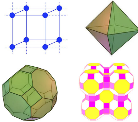
Figure 2: An example F(X) , when X is the cubic lattice (top left). Each link graph is an octahedron (top right), and so each pineapple of F(X) is a truncated cuboctahedron (bottom left). The pineapples are arranged as in the bottom right figure, which shows four of them in the front.
