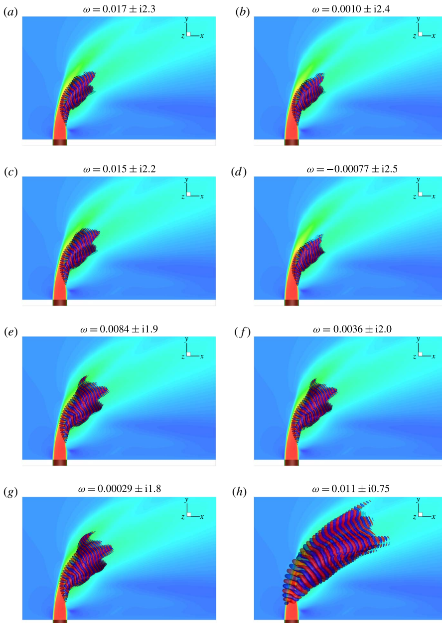
FIGURE 12. (Colour online) Real part of the eigenmodes for case R4 are shown with positive and negative isocontours of \tilde{u} and \bar{v} contours of the base state in the background to highlight the jet base flow. The associated eigenvalues are shown above, with the real part being the growth rate and the imaginary part being the Strouhal number. Modes (a–g) correspond to the higher-frequency downstream shear-layer modes. Mode (h) is associated with the upstream shear layer.
